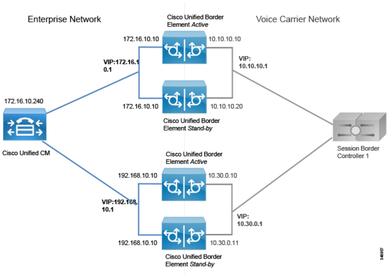
図 4-24 複数の Cisco Unified Border Element
