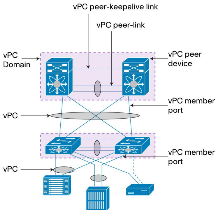
Figure 2. vPC Components
