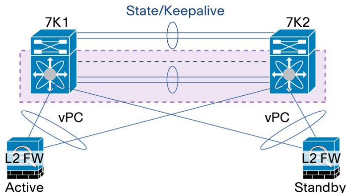
Figure 72. Network Services Appliance Configured in Transparent Mode Connected to vPC Domain
