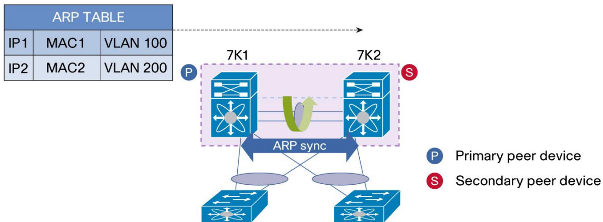
Figure 93. vPC ARP Sync - vPC Peer-Link Fails and Recovers
