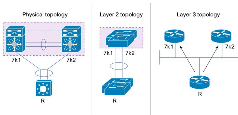
Figure 49. Different Views for vPC Peer Devices Depending on Layer 2 or Layer 3 Vision of the Network
