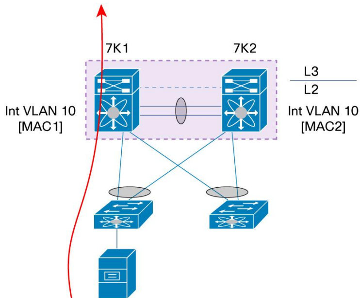
Figure 91. vPC Peer-Gateway
