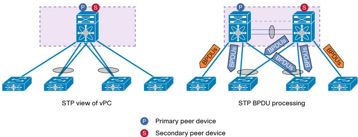
Figure 44. STP BDPUs Processing with vPC Peer-Switch
