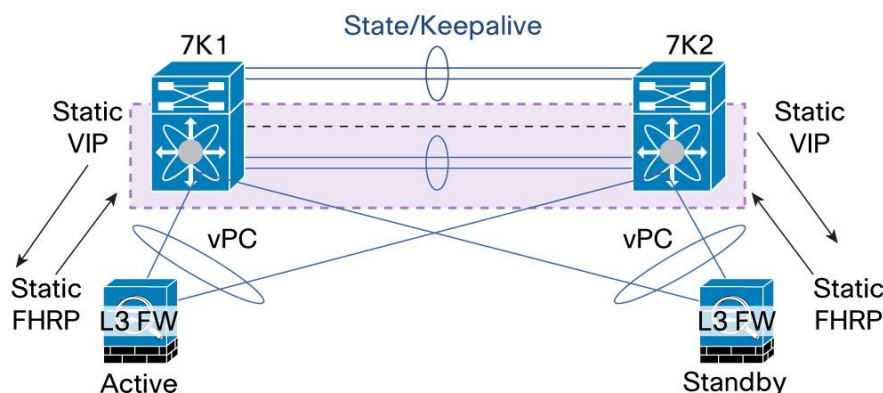
Figure 75. Service Appliance in Routed Mode Connected to vPC Domain Using vPC Link
