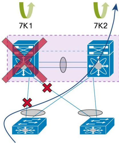
Figure 97. vPC Auto-Recovery Reload-Delay - Both vPC Peer Devices Reload But Only 7K2 Comes Back to Life
