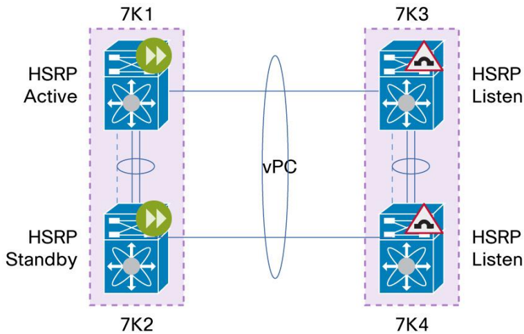
Figure 68. DC1 with a Single HSRP/VRP Group - Active/Active in DC1 and Listen/Listen in DC2
