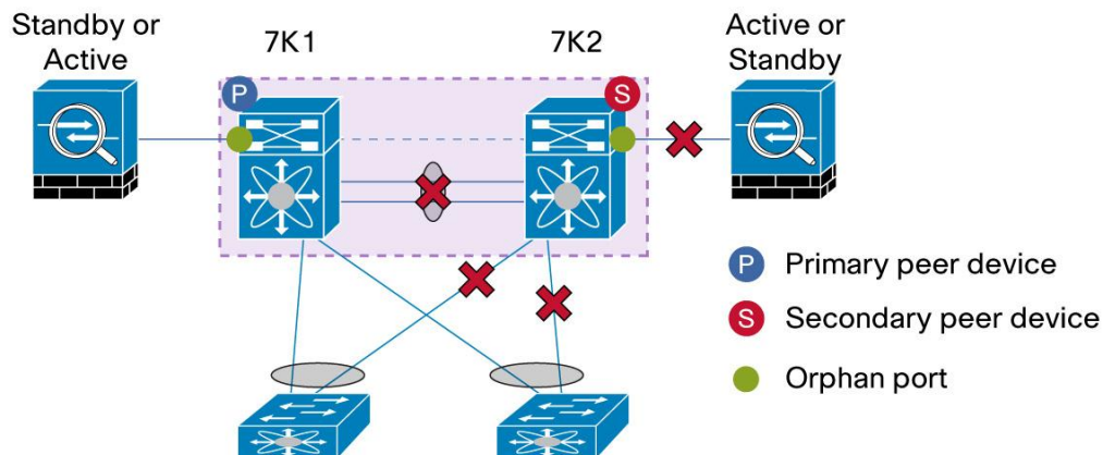
Figure 98. vPC Orphan Ports Suspend
