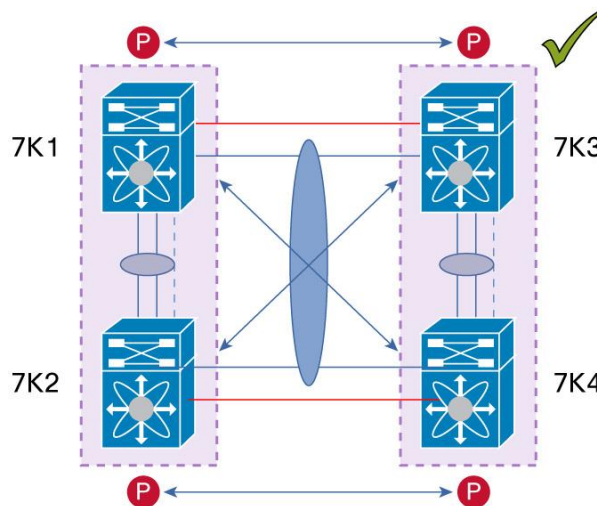
Figure 58. Layer 3 and vPC Supported Designs: Peering over a vPC Interconnection (DCI case) on Parallel Interconnected Routed Ports
