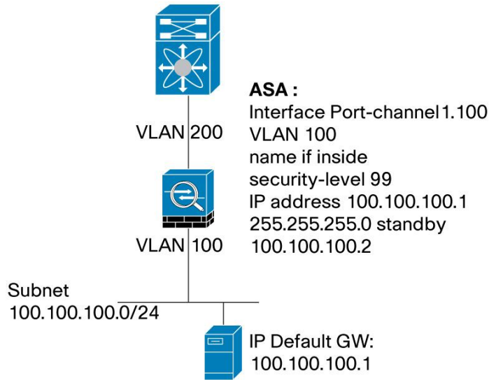
Figure 78. ASA in Routed Mode Connected to vPC Domain - Logical View
