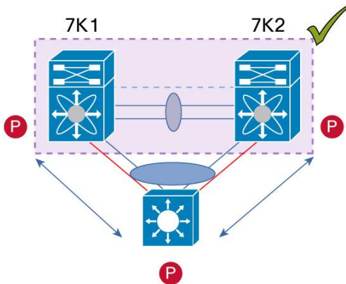
Figure 57. Layer 3 and vPC Supported Designs: Peering with an External Router on Parallel Interconnected Routed Ports
