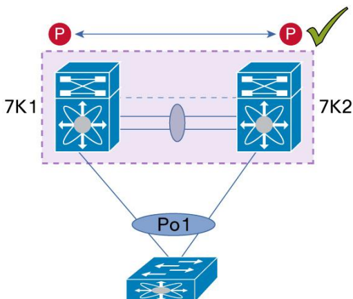
Figure 54. Supported Designs for Layer 3 and vPC: Peering Between vPC Devices (for Backup Routing Path)
