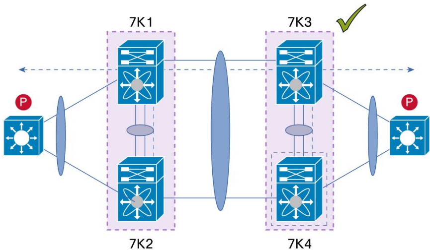
Figure 56. Layer 3 and vPC Supported Designs: Peering between Two Routers with vPC Devices as Transit Switches
