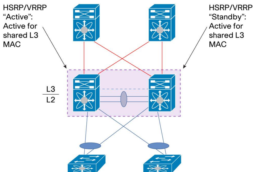
Figure 66. HSRP/VRRP Active-Active with vPC
