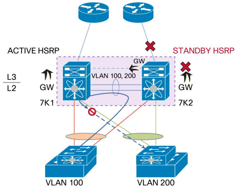
Figure 67. The Problem with HSRP/VRRP Object Tracking in a vPC Configuration
