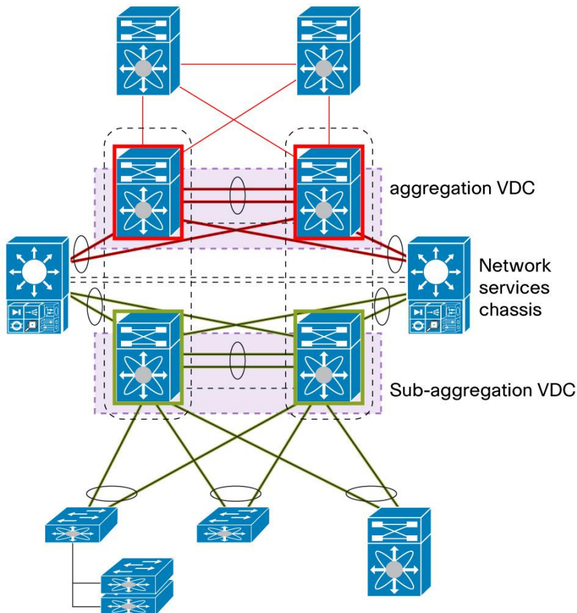
Figure 71. Network Services Chassis with VDC Sandwich Design
