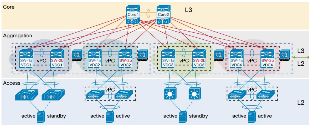
Figure 86. vPC and VDC Interaction - Creating 4 Independent vPC Domains with 2 NEXUS 7000 Series Chassis
