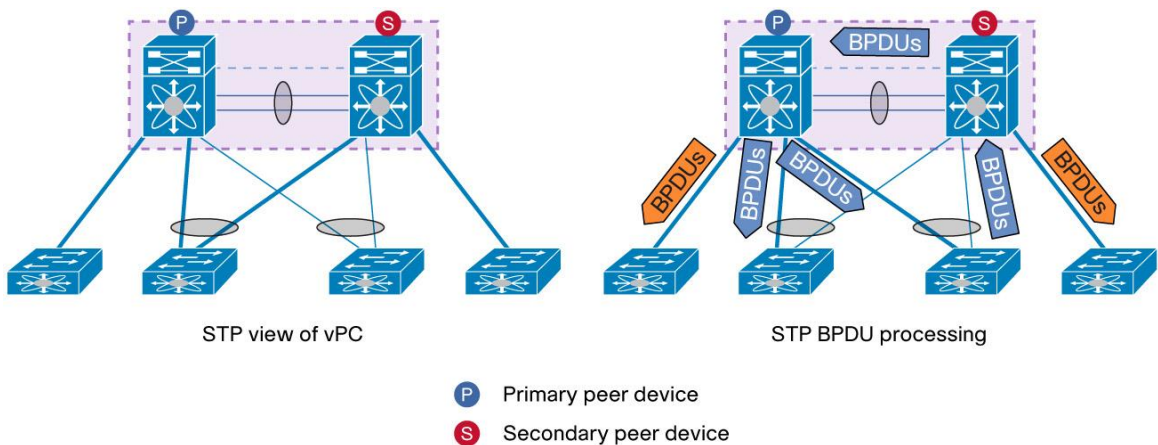
Figure 43. STP BDPUs Processing without vPC Peer-Switch
