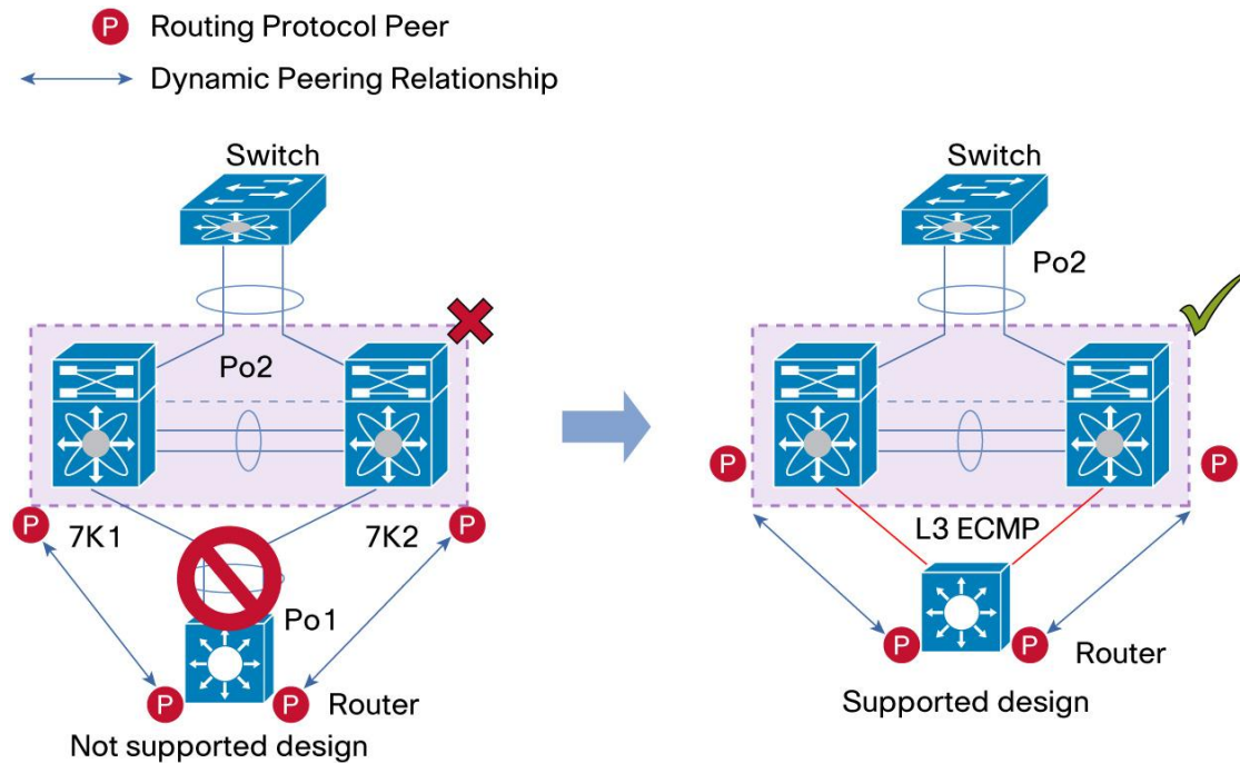
Figure 50. Using Separate Layer 3 Links to Connect L3 Device to a vPC Domain
