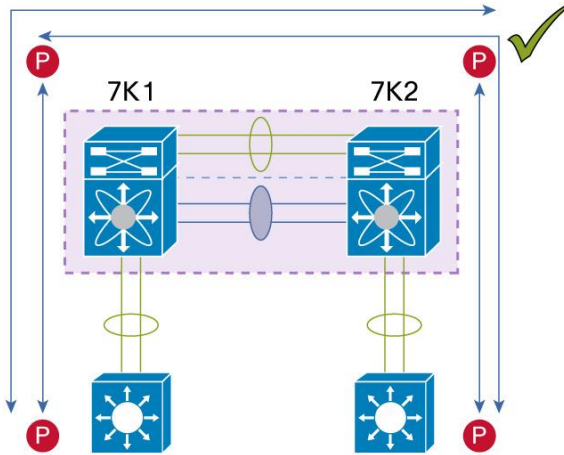
Figure 59. Layer 3 and vPC Supported Designs: Peering over PC Interconnection and Dedicated Interswitch Link Using non-vPC VLAN
