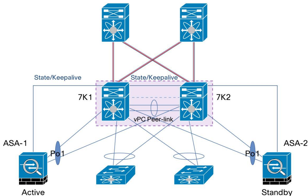
Figure 77. ASA Services Appliance Configured in Routed Mode and Connected to vPC Domain
