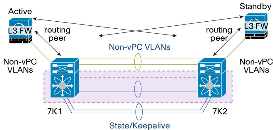
Figure 76. Service Appliance in Routed Mode Connected to vPC Domain Using Single Link
