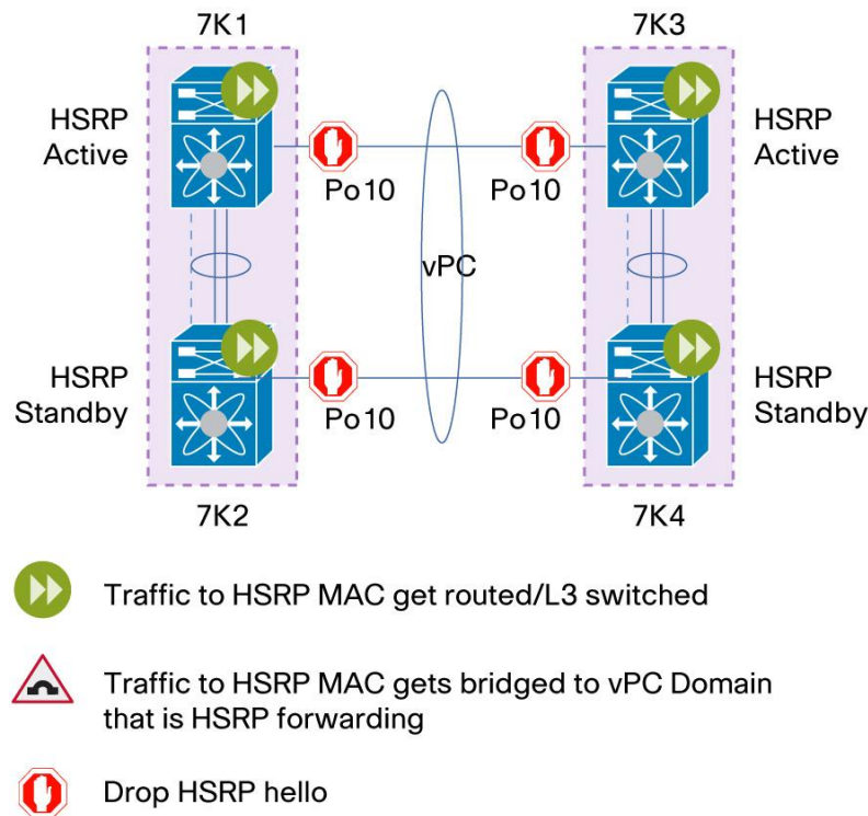
Figure 70. DCI with a Single HSRP/VRRP Group - Active/Active in DC1 and Active/Active in DC2
