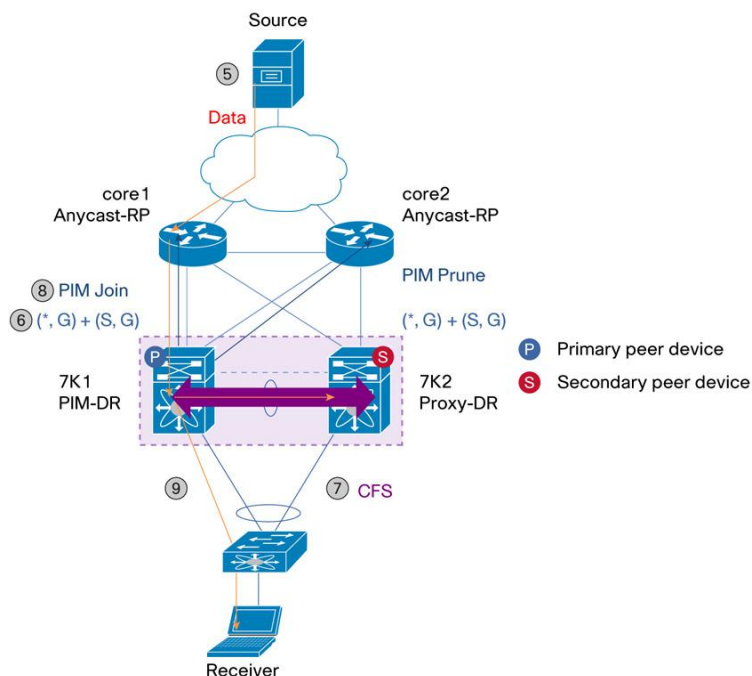
Figure 81. How Multicast Works with vPC (Multicast Packet Flow) - Contd
