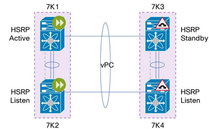
Figure 69. DCI with a Single HSRP/VRP Group - Active/Active in DC1 and Listen/Listen in DC2
