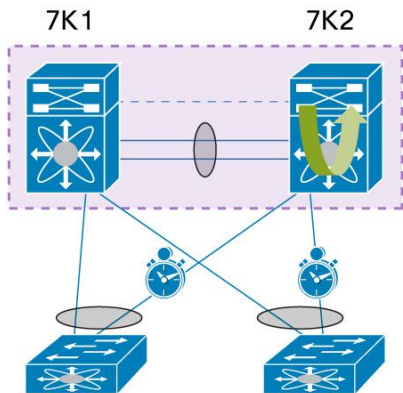
Figure 94. vPC Delay Restore - 7K2 Fails and Then Recovers
