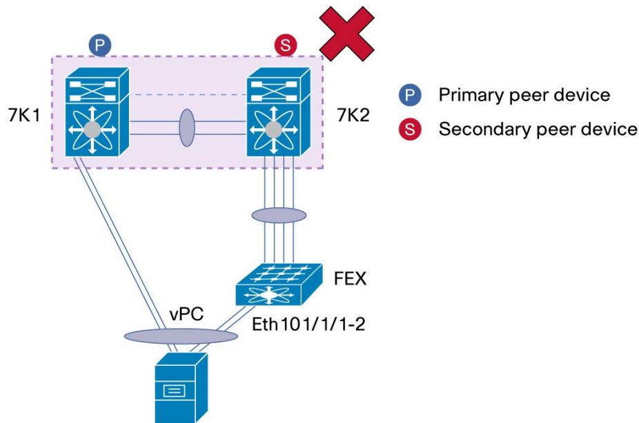
Figure 85. FEX with vPC - vPC with 1 Leg on FEX and the Other Leg On NEXUS 7000 Line Card - Not Supported
