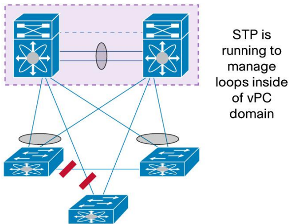
Figure 39. Role of STP within vPC Domain
