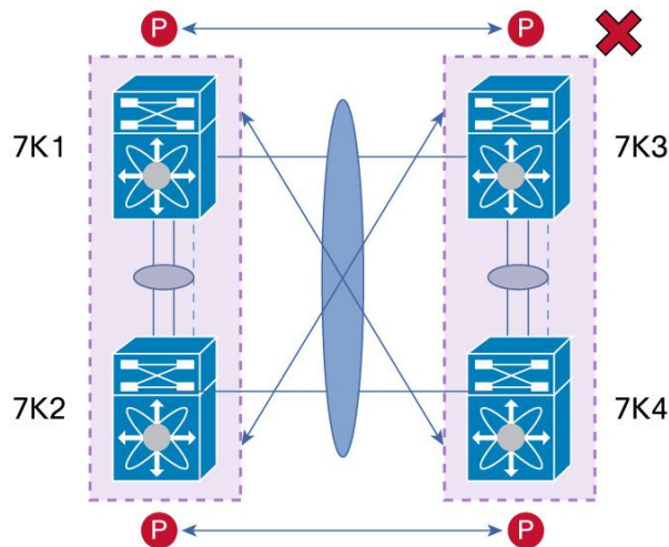
Figure 63. Layer 3 and vPC Unsupported Designs: Peering Over a vPC Interconnection (DCI Case)
