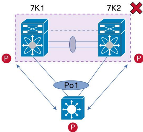
Figure 61. Layer 3 and vPC Unsupported Designs: Peering Over a vPC Interconnection
