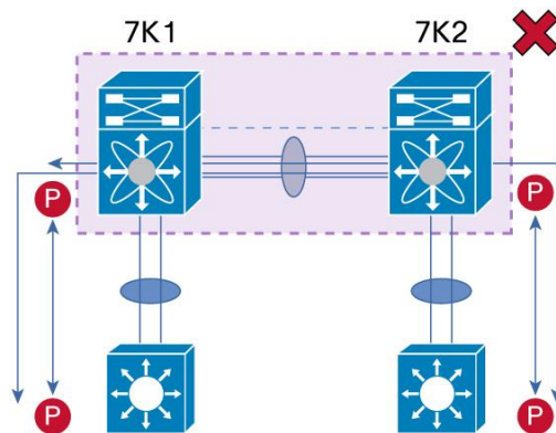
Figure 64. Layer 3 and vPC Unsupported Designs: Peering Over PC Interconnection and Over vPC Peer-Link Using vPC VLAN
