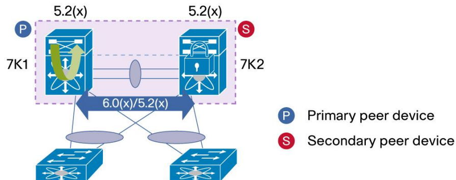
Figure 88. ISSU with vPC - Step 1
