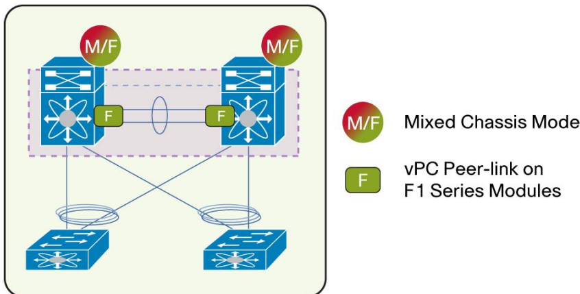
Figure 92. vPC Peer-Gateway Exclude-VLAN - Unique Topology Where the Feature Apply
