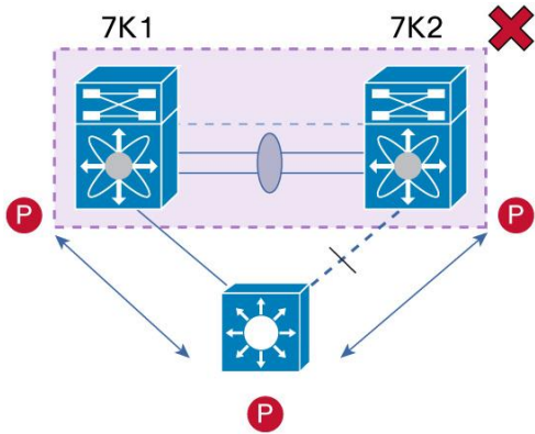
Figure 62. Layer 3 and vPC Unsupported Designs: Peering Over a Spanning Tree Protocol Interconnection Using a vPC VLAN
