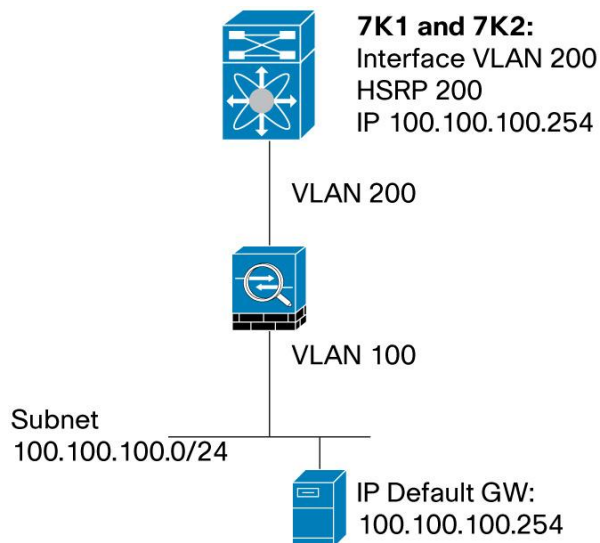
Figure 74. ASA in Transparent Mode Connected to vPC Domain - Logical View
