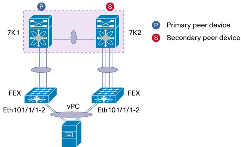
Figure 83. FEX with vPC - Host vPC
