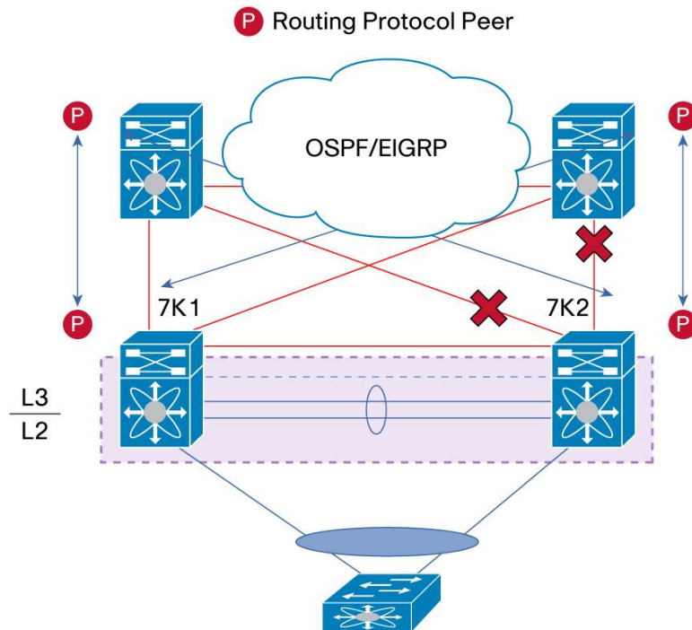
Figure 65. Establishing a L3 Backup Routing Path Between vPC Peer Devices
