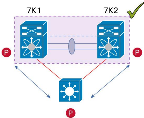
Figure 53. Supported Designs for Layer 3 and vPC: Peering with an External Router Using L3 Links
