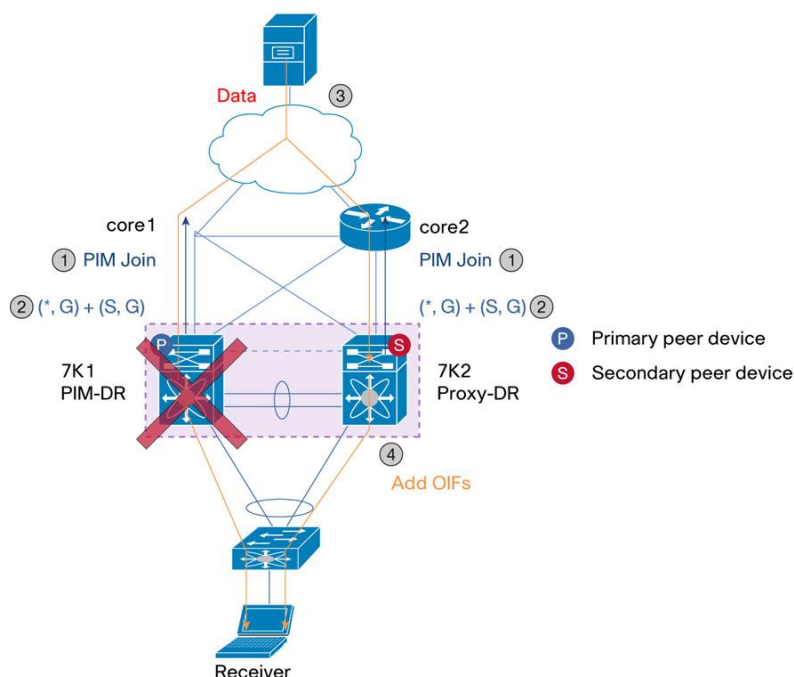
Figure 82. Multicast with vPC - PIM Prebuild SPT
