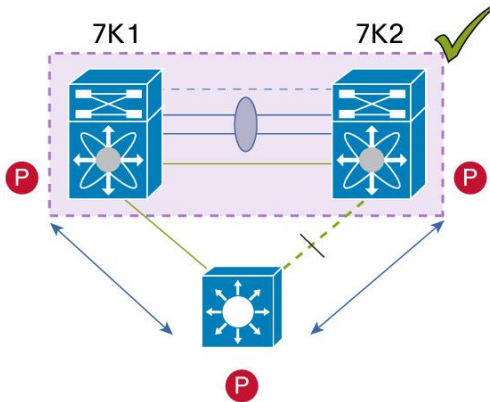
Figure 55. Supported Designs for Layer 3 and vPC: Peering over a Spanning Tree Protocol Interconnection Using a non-vPC VLAN
