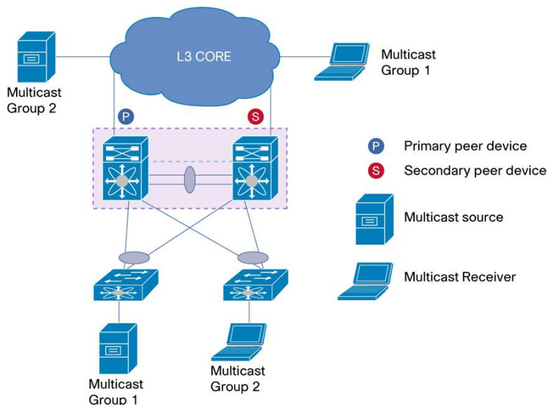
Figure 79. Multicast with vPC
