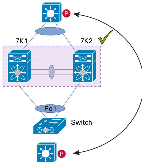
Figure 52. Supported Designs for Layer 3 and vPC: Peering Between ROUTERS
