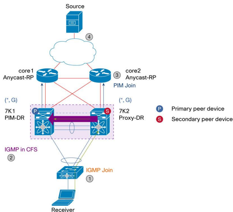
Figure 80. How Multicast Works with vPC (Multicast Packet Flow)
