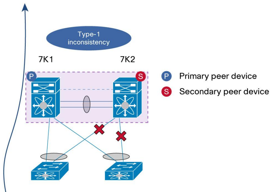
Figure 95. vPC Graceful Type-1 Checks
