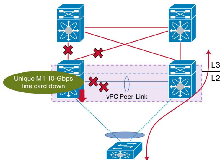
Figure 21. vPC Object Tracking Feature - Behavior When vPC Peer-Link Fails Down
