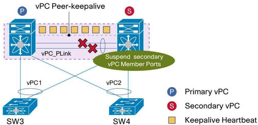
Figure 11. vPC Peer-Link Failure - Behavior On Secondary Peer Device
