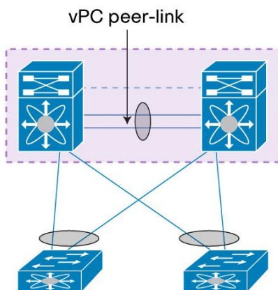
Figure 17. vPC Peer-Link
