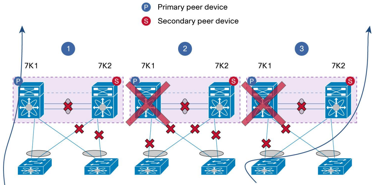
Figure 96. vPC Auto-Recovery - vPC Peer-Link Failure Then vPC Primary Peer Device Failure
