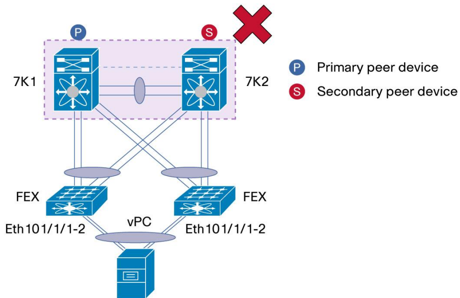
Figure 84. FEX with vPC - eVPC (Enhanced vPC) - Not Supported
