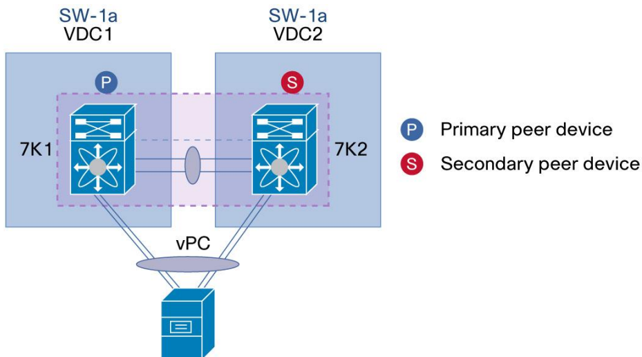
Figure 87. vPC Domain Created Within the Same NEXUS 7000 Chassis Using 2 Different VDC
