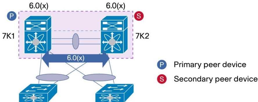
Figure 90. ISSU with vPC - Step 3
