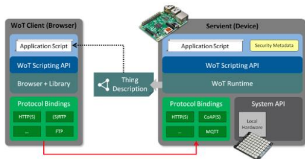
Servient on Device Itself
