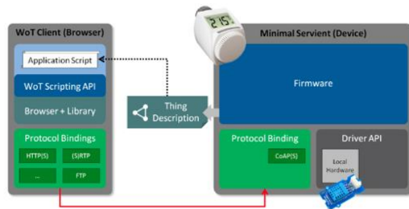
Resource-constrained Device as Thing
