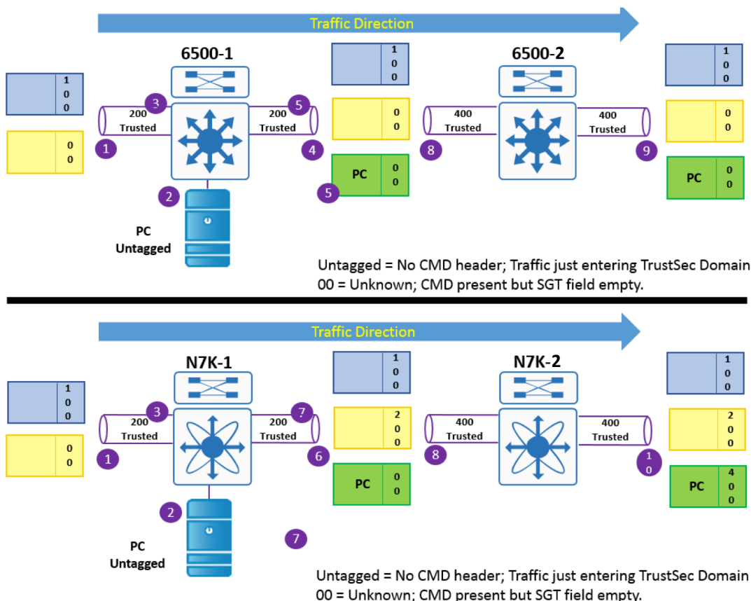
Figure 11 Behavior for policy static trusted on Catalyst and Nexus switches
