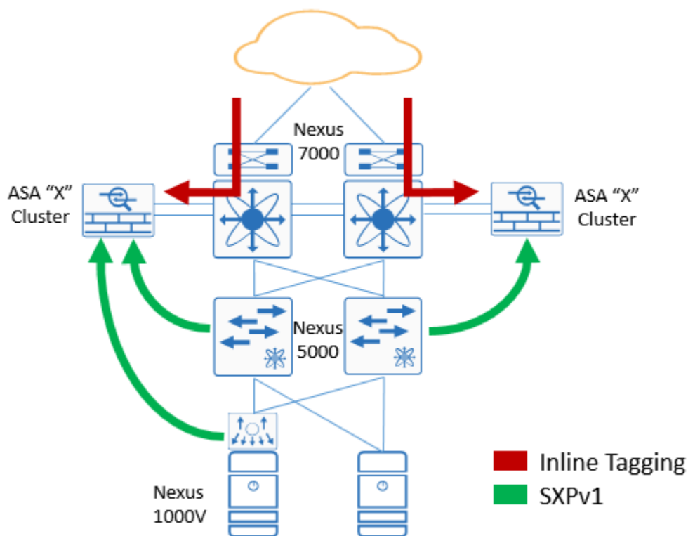
Figure 8 Inline tagging used with SXP
