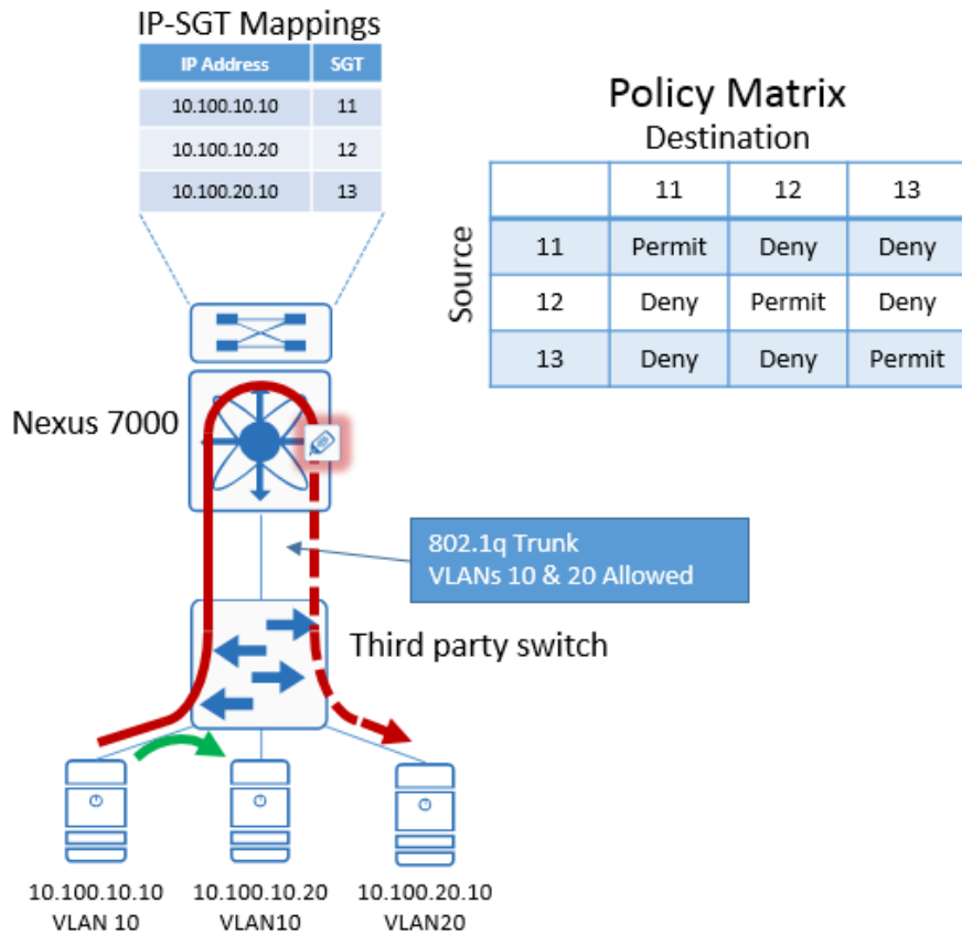
Figure 25 Nexus 7000 using IP-SGT mappings for enforcement
