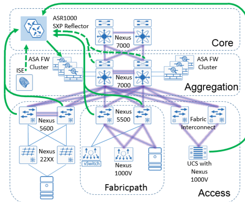
Figure 60 TrustSec propagation in the sample Data Center
