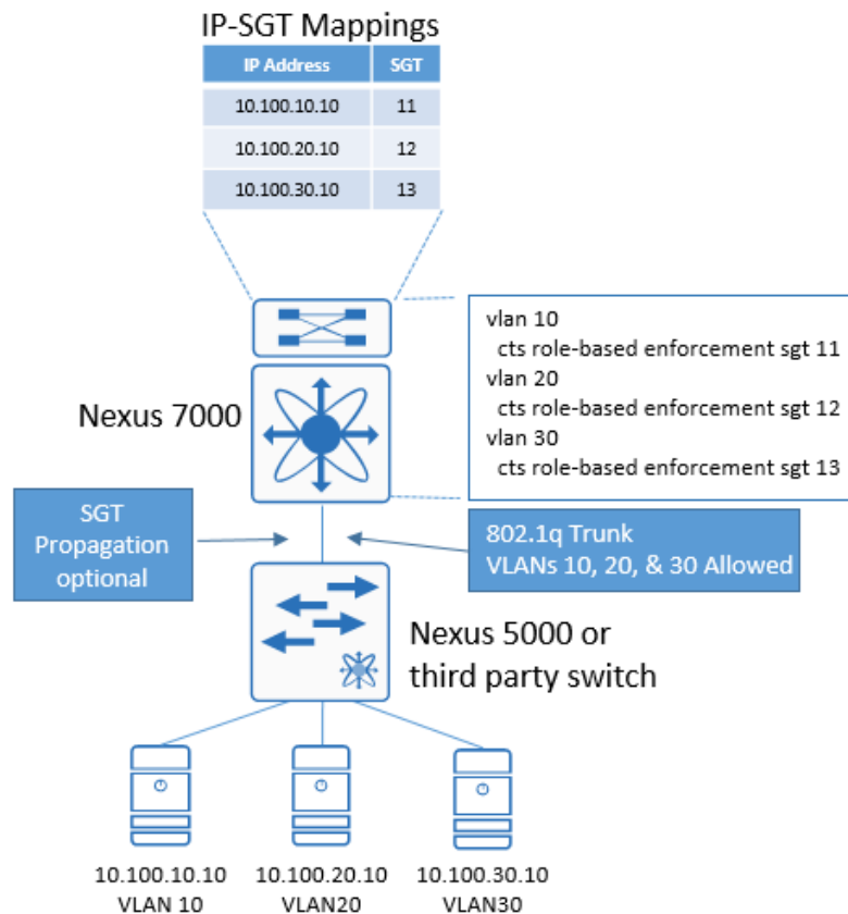
Figure 27 Nexus 7000 and VLAN-SGT mapping
