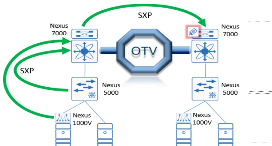
Figure 15 SXP over OTV between data centers
