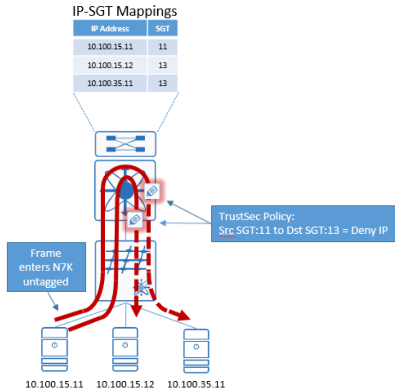
Figure 26 Nexus 7000 using static IP-SGT mapping with FEX
