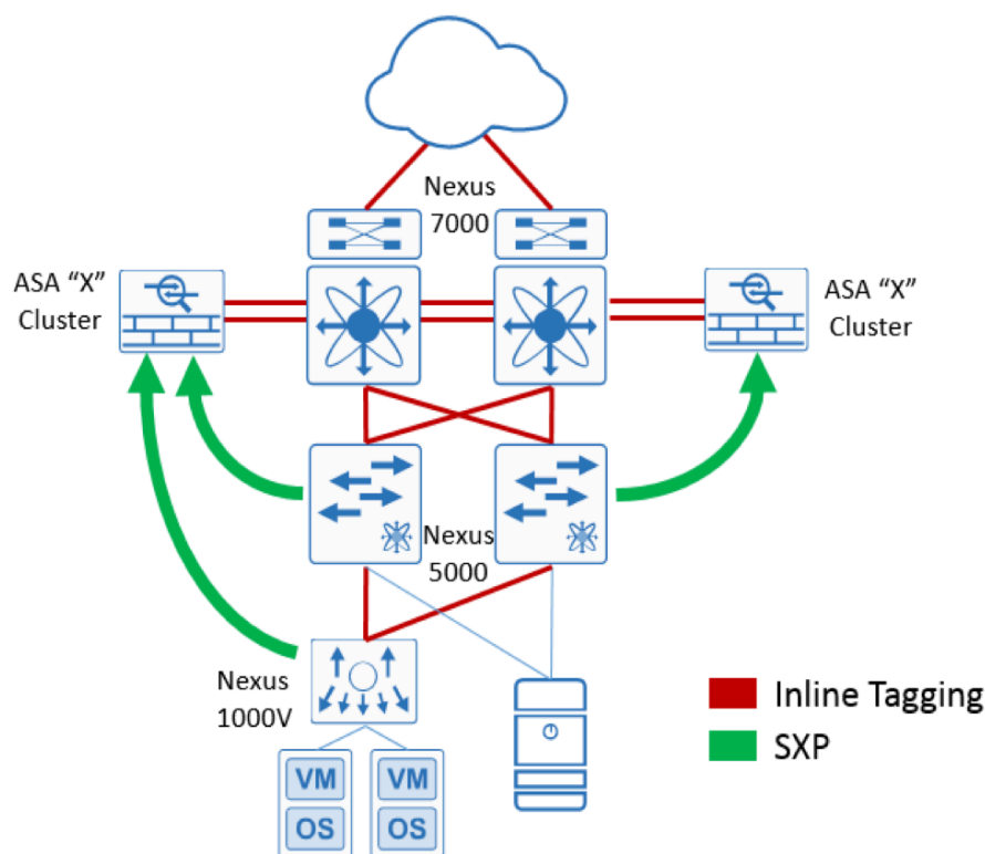
Figure 29 ASA SGFW using SXP and inline tagging
