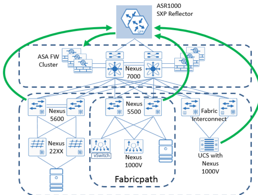
Figure 13 SXP Reflector aggregating SXP advertisements
