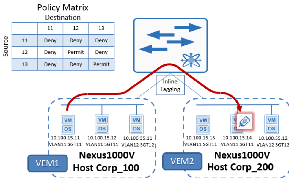
Figure 20 Nexus 1000 and TrustSec policy enforcement across L2 VDS
