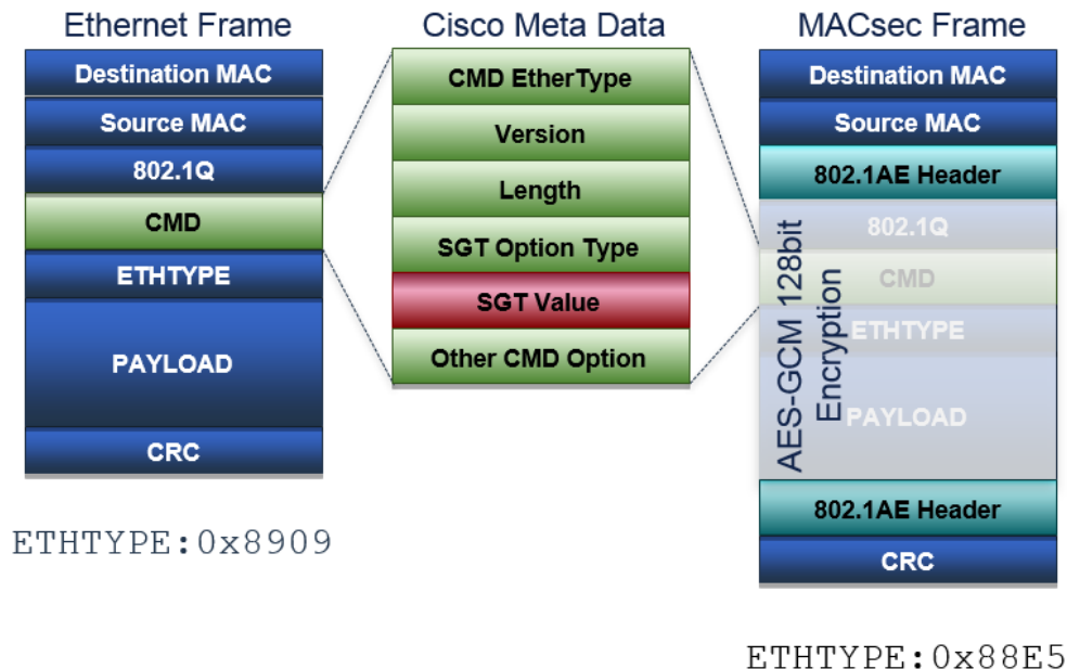
Figure 2 Comparison of Ethernet and MACsec 802.1AE frames carrying Cisco MetaData
