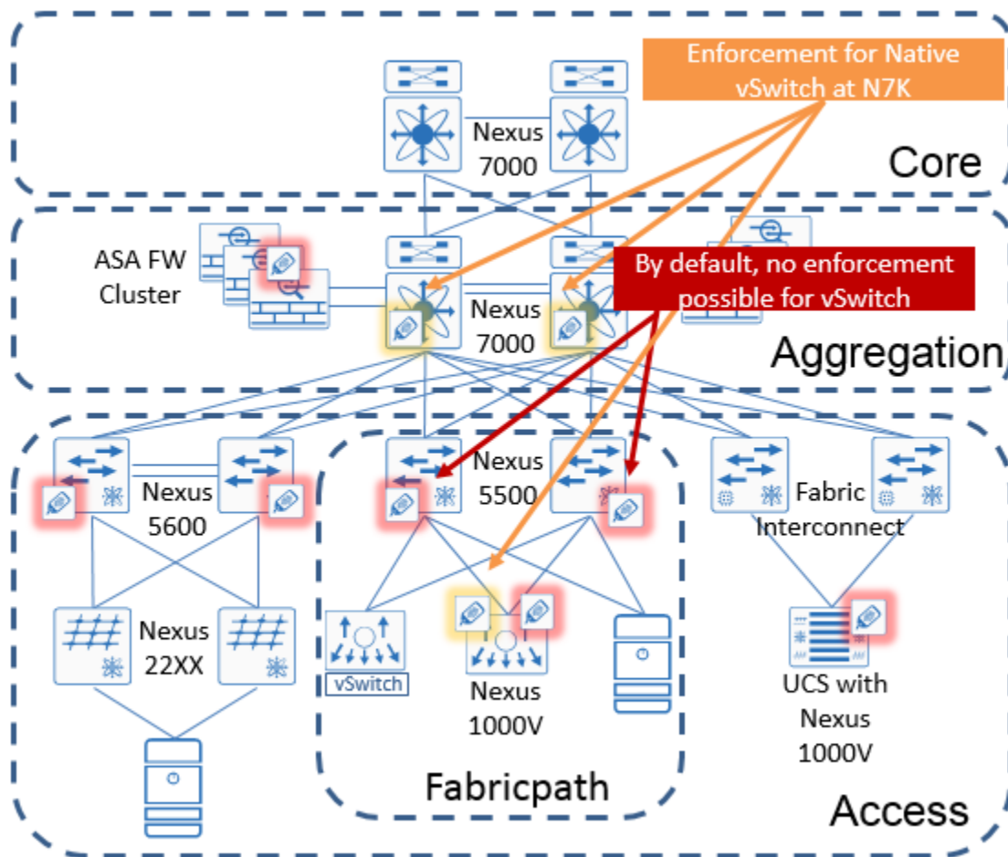
Figure 18 Default points of enforcement
