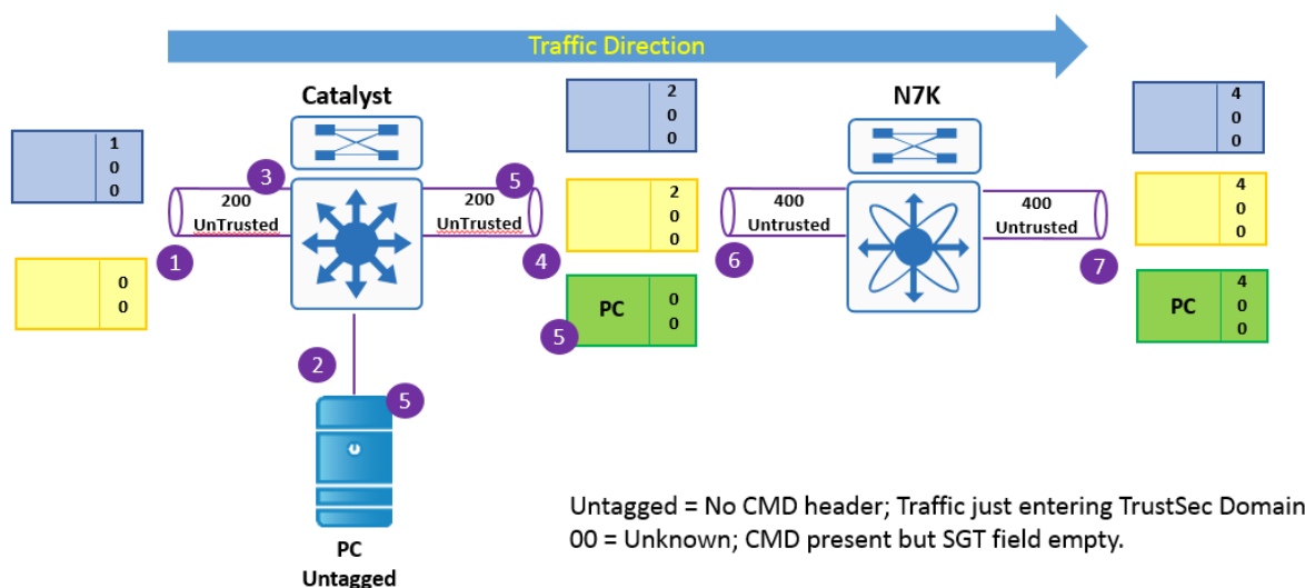
Figure 10 Behavior for policy static untrusted on Catalyst and Nexus switches
