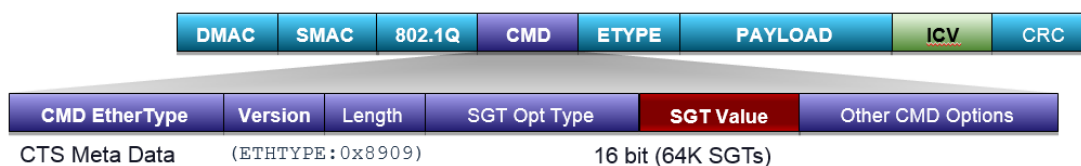
Figure 1 Layer 2 Frame with Cisco Meta Data field containing SGT
