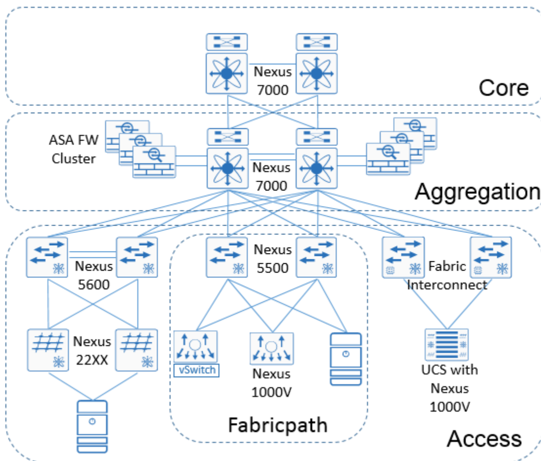
Figure 3 Data Center Example
