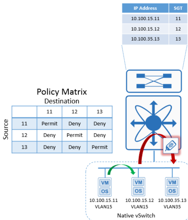
Figure 31 TrustSec enforcement for Virtual Servers on native vSwitch
