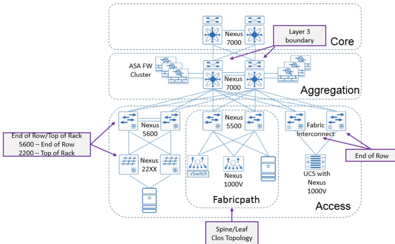
Figure 23 Data Center topologies
