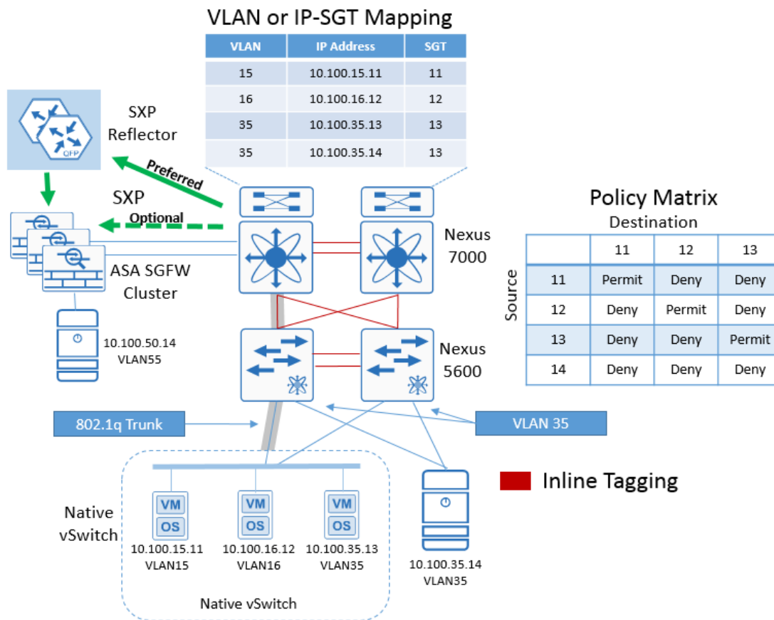
Figure 35 Native vSwitch enforcement at SGFW
