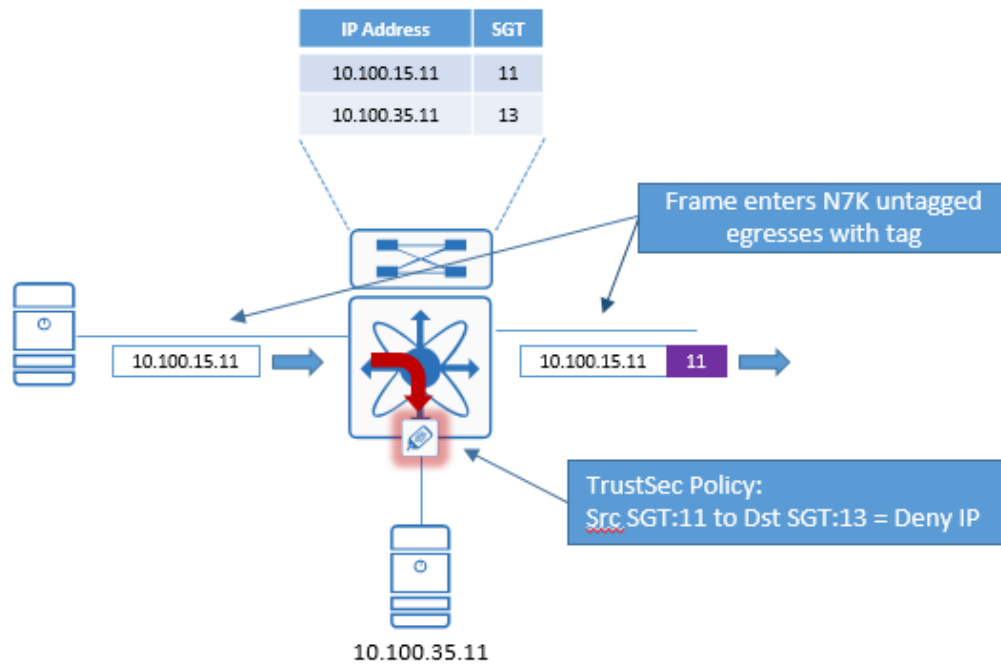
Figure 24 Nexus 7000 using static IP-SGT mapping
