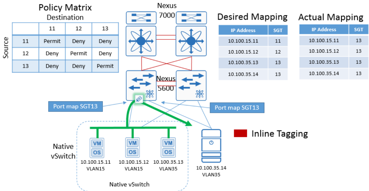
Figure 32 Native vSwitch connected to Nexus 5600
