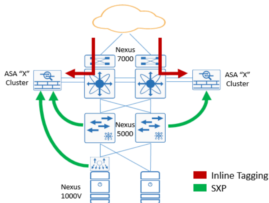
Figure 16 SXP use with ASA Cluster in the data center
