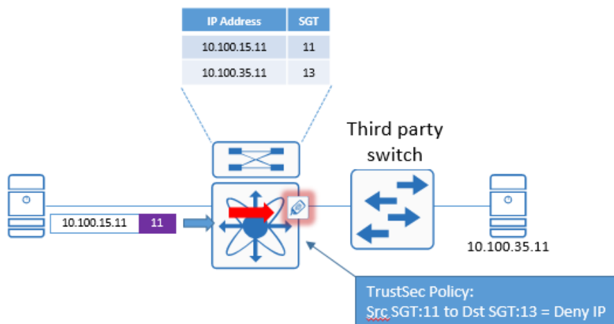
Figure 6 Static IP-SGT mapping used for enforcement
