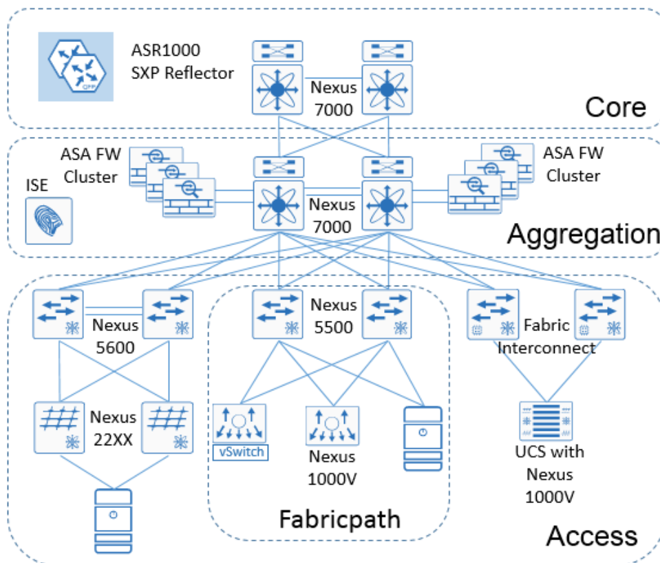
Figure 36 Sample Data Center infrastructure
