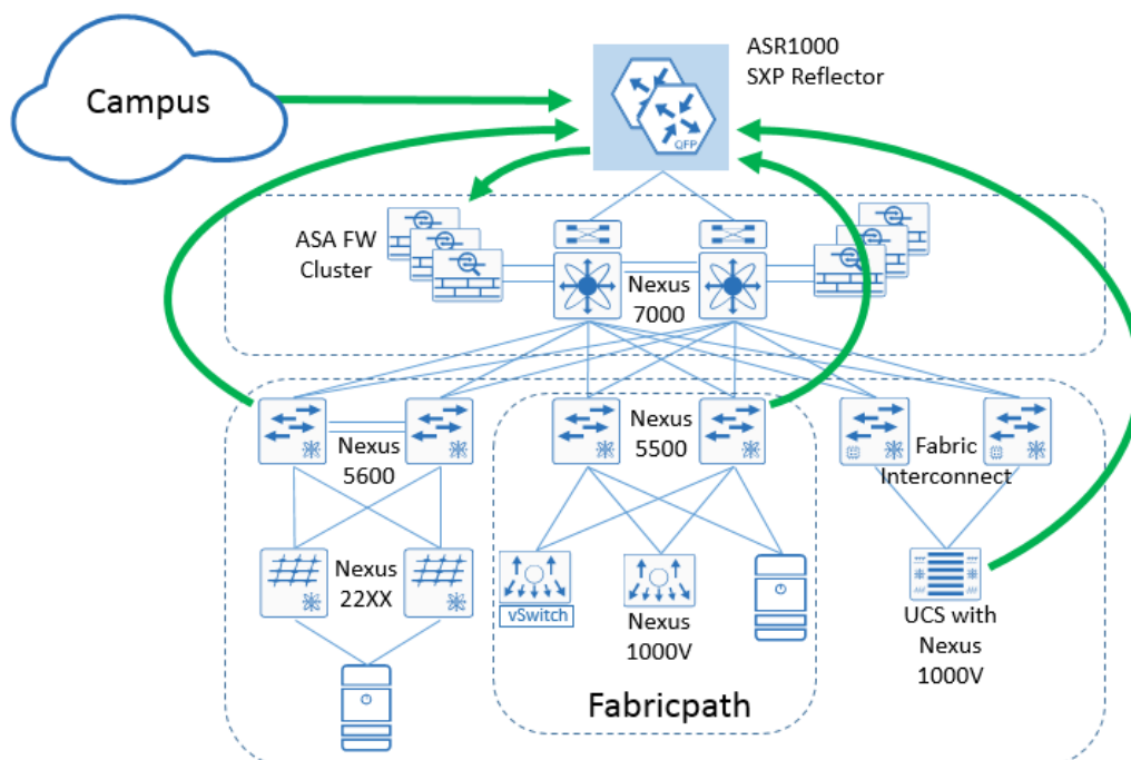
Figure 30 SXP Reflector aggregating SXP advertisements for the ASA
