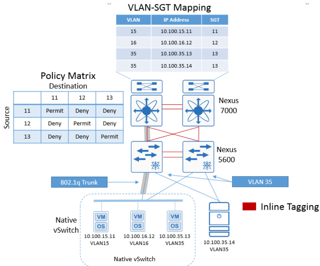
Figure 34 Native vSwitch using VLAN-SGT at Nexus 7000
