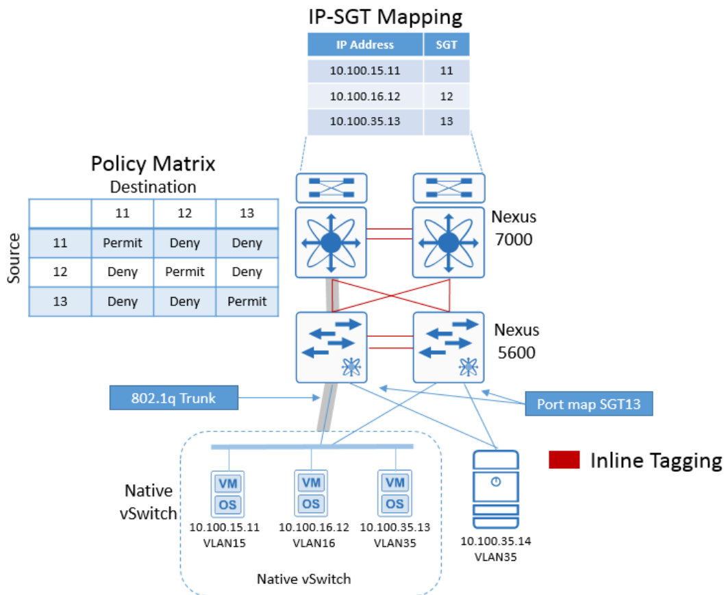
Figure 33 Native vSwitch using IP-SGT at Nexus 7000
