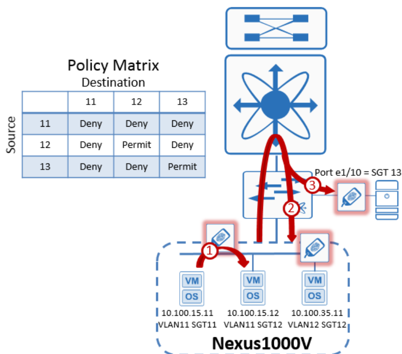
Figure 19 Nexus 1000V and TrustSec policy enforcement
