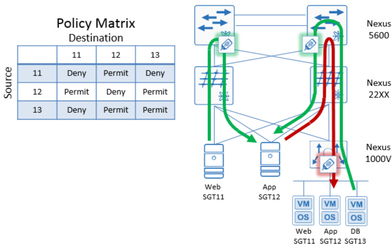
Figure 22 Nexus 5000 Port Level Enforcement
