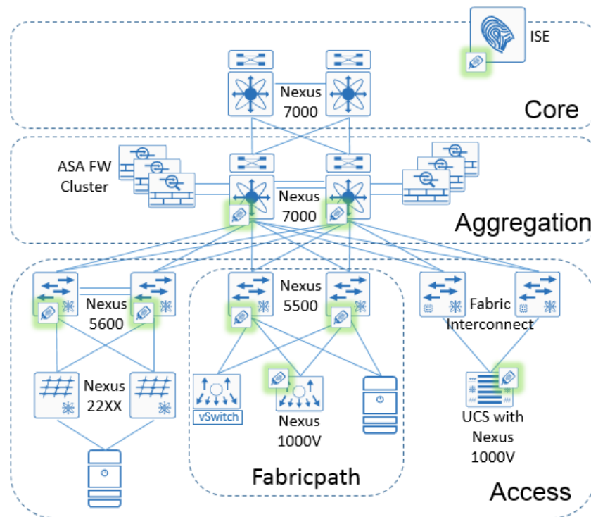
Figure 4 Classification in the data center
