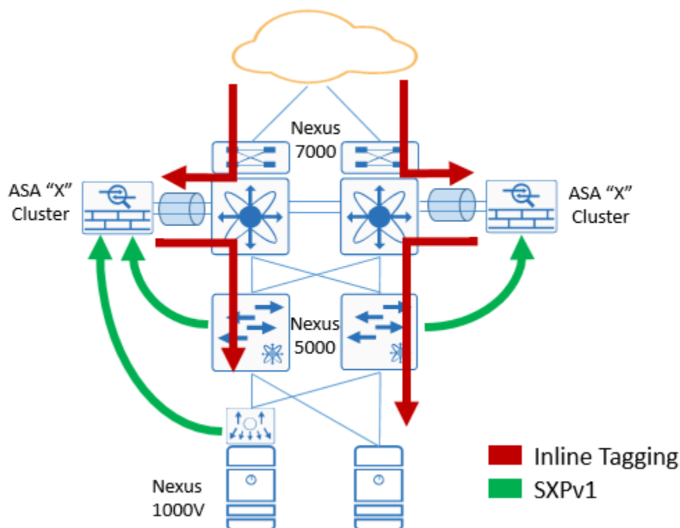
Figure 9 Inline tagging on a trunk to ASA with SXP
