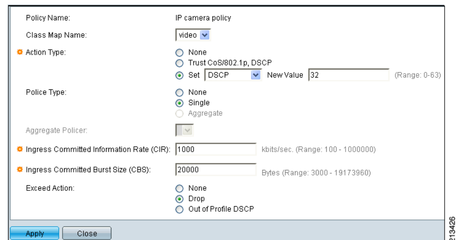
Figure 16 Adding Policing/Marking Actions
