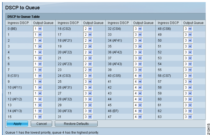
Figure 5 DSCP to Queue Screen
