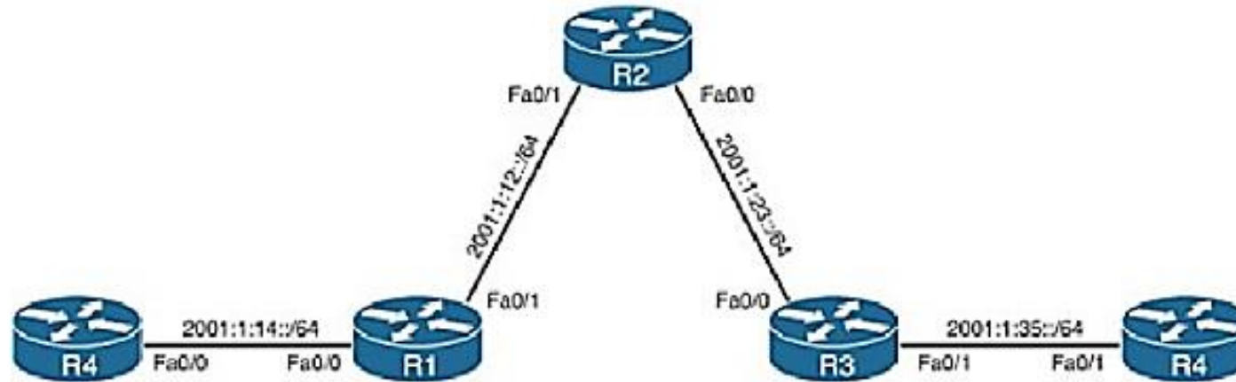
IPv6 Multicast Topology
