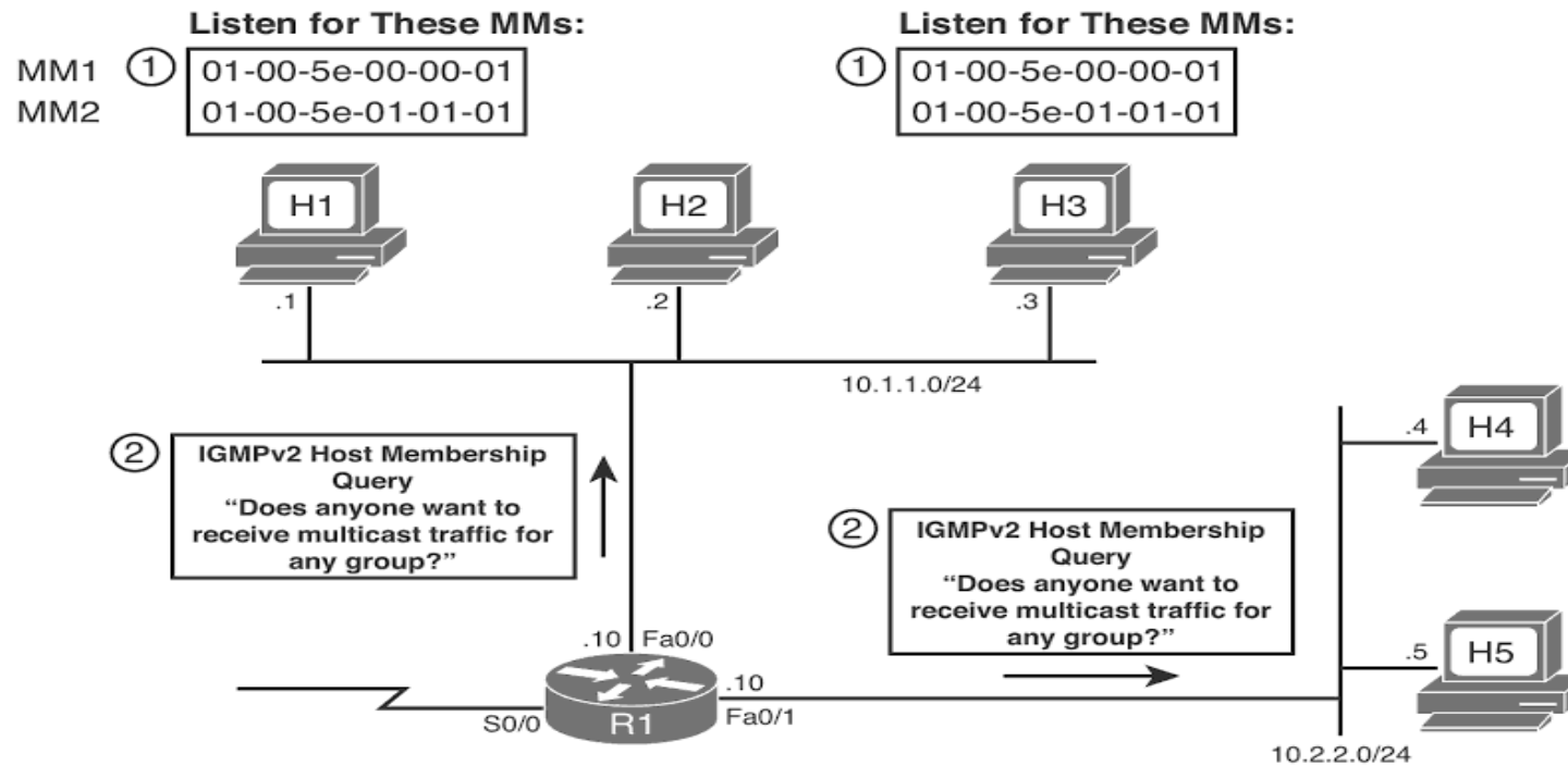
IGMPv2 Host Membership Query Process
