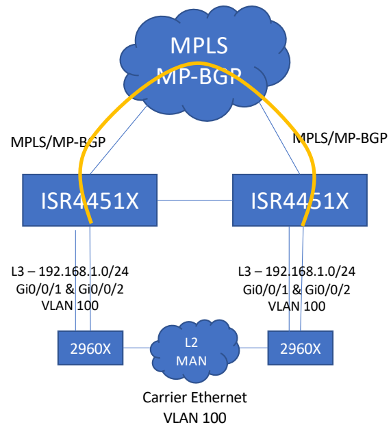
Backup of MAN via MPLS L2VPN
