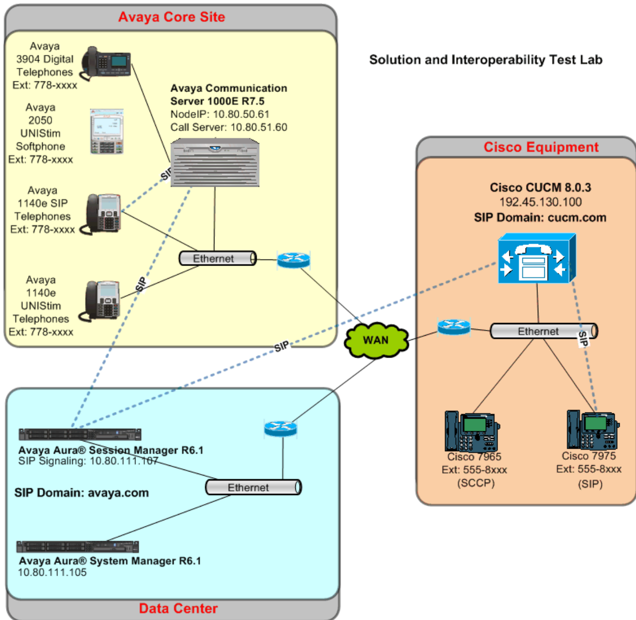
Figure 1 – Sample Configuration
