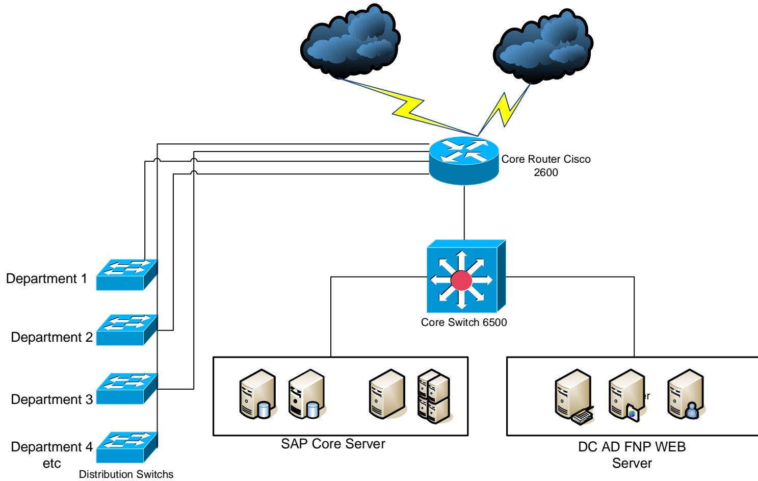
Core Network Diagram Simplified
