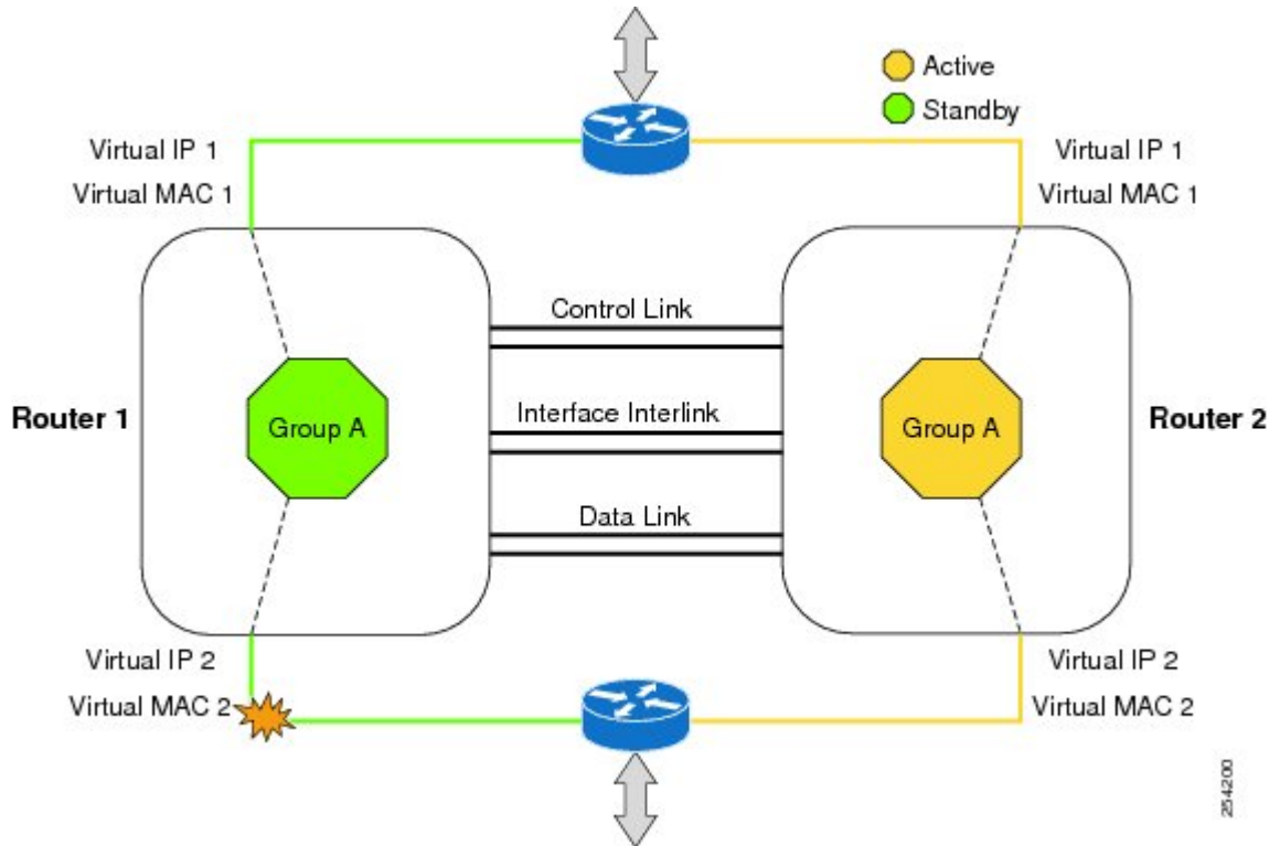
Figure 1: Redundancy Group Configuration—One Outgoing Interface
