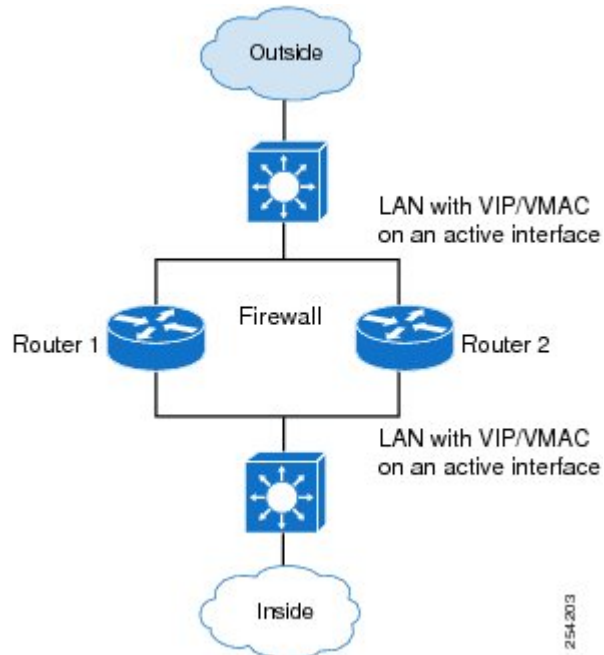
Figure 2: LAN-LAN Topology
