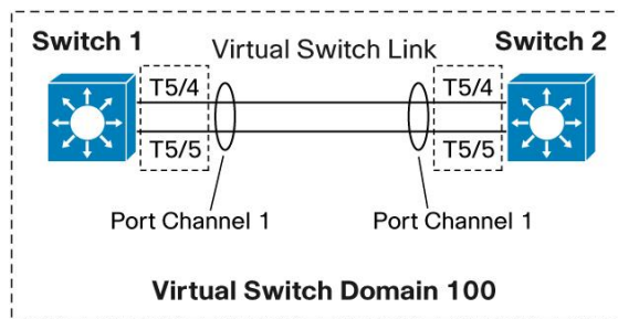
Figure 11. Cisco Virtual Switching System Conversion
