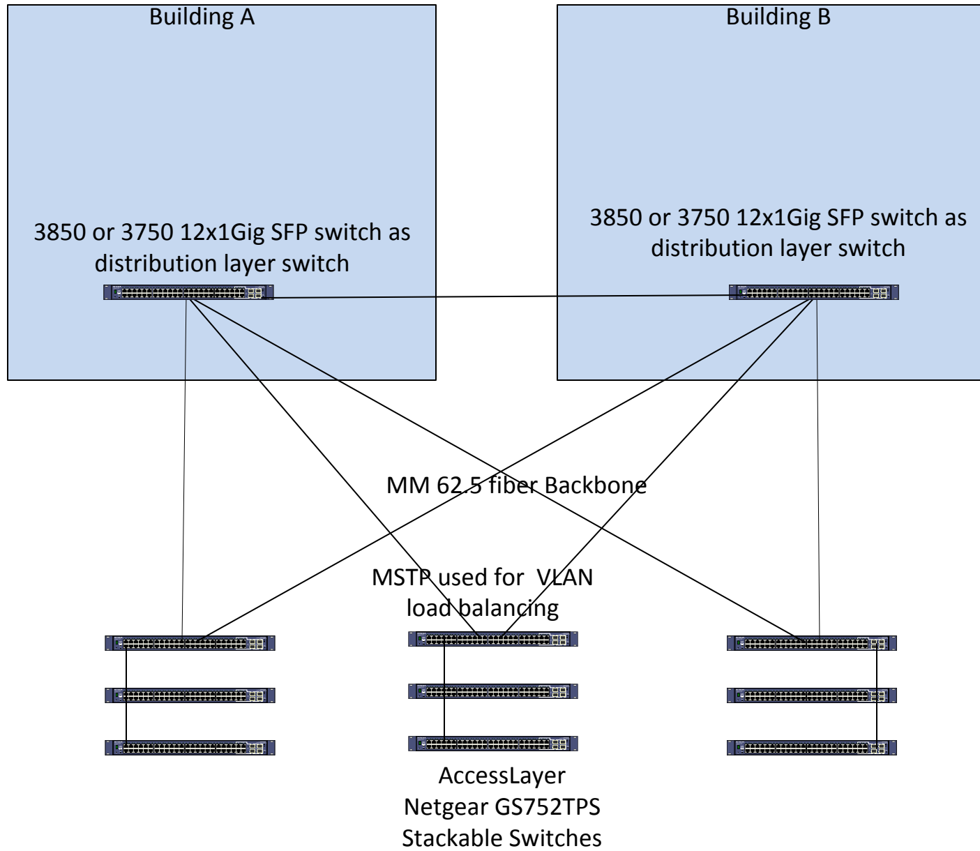
Standalone Dist layer switches using STP,HSRP for Layer 2 and Layer 3 resilience
