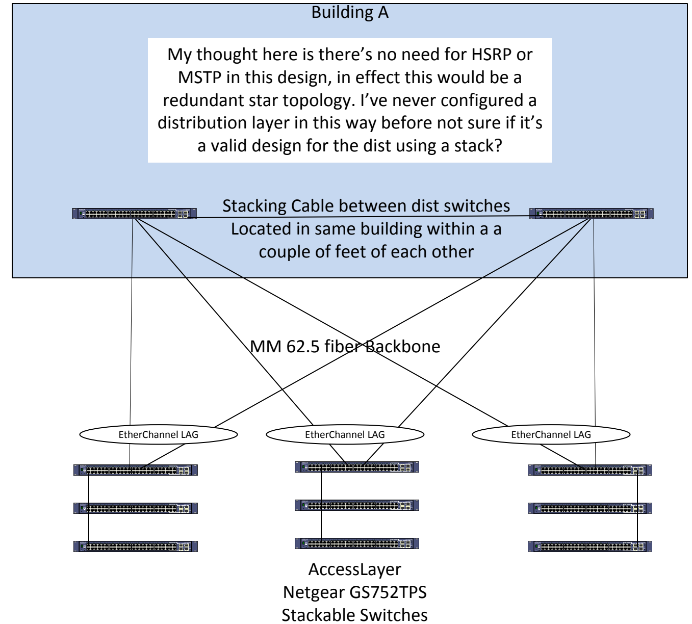
Standalone Dist layer switches using STP,HSRP for Layer 2 and Layer 3 resilience
