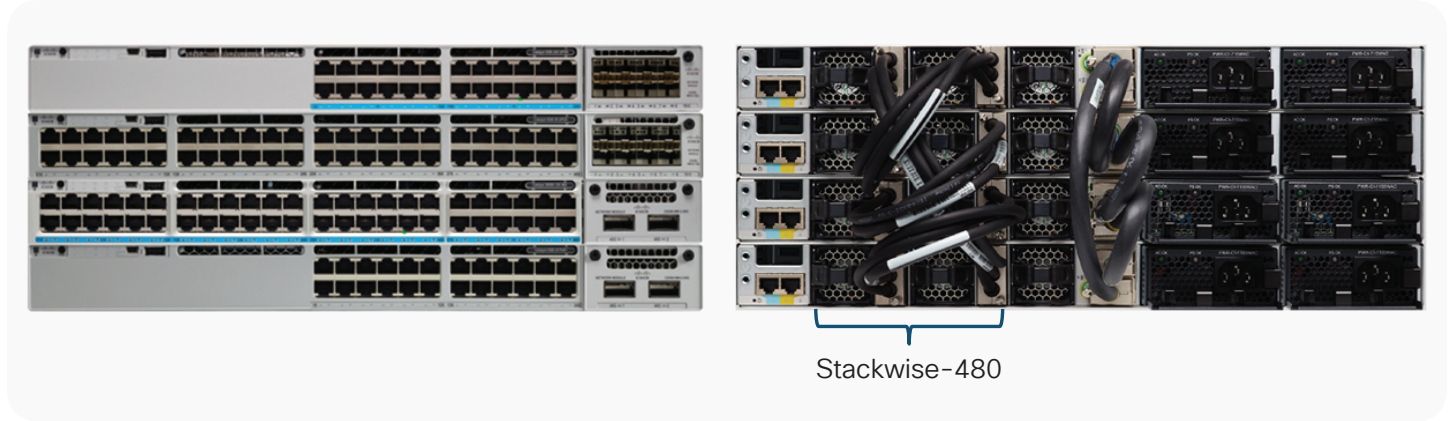
Figure 1. Cisco Catalyst 9300 Series StackWise-480 technology
