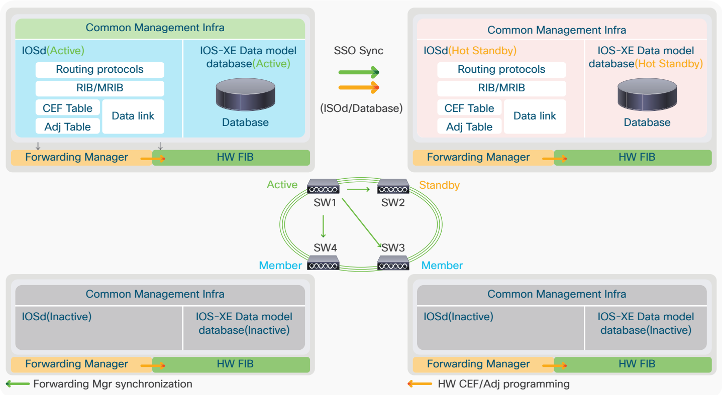
Figure 7. Cisco Catalyst 9300 Series and centralized processing
