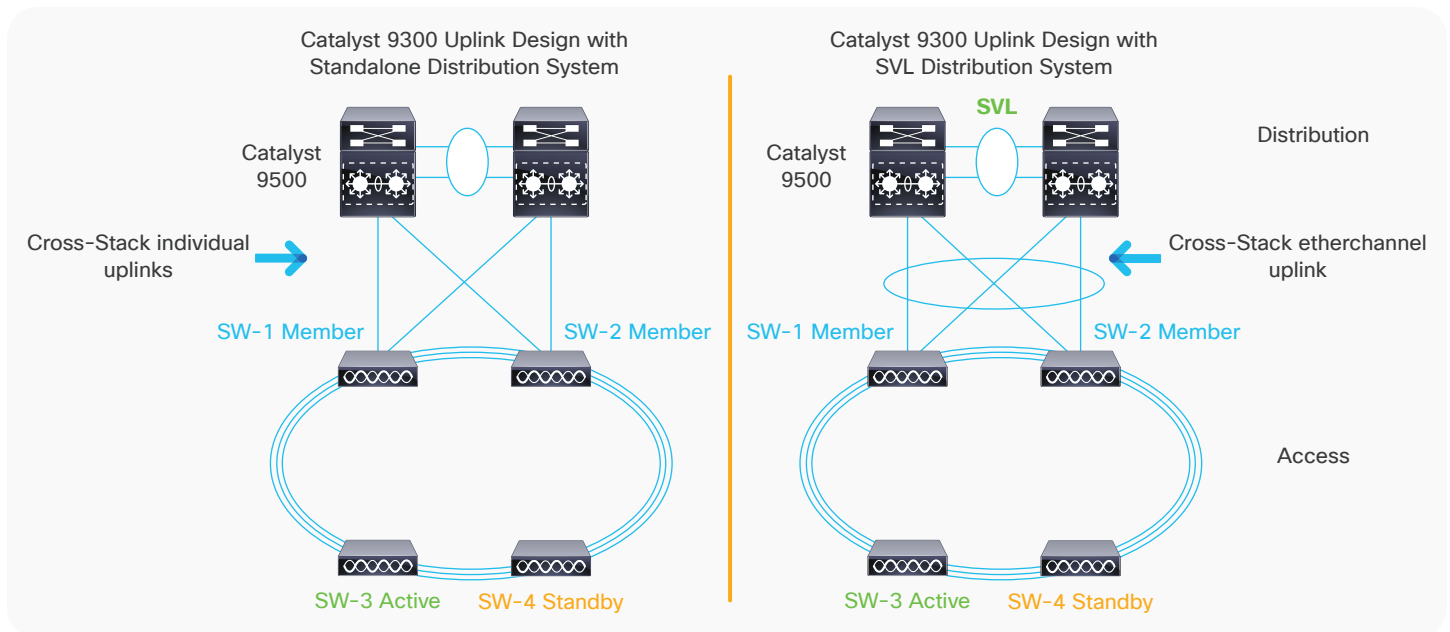
Figure 17. Cisco Catalyst 9300 Series StackWise-480 uplink design best practices
