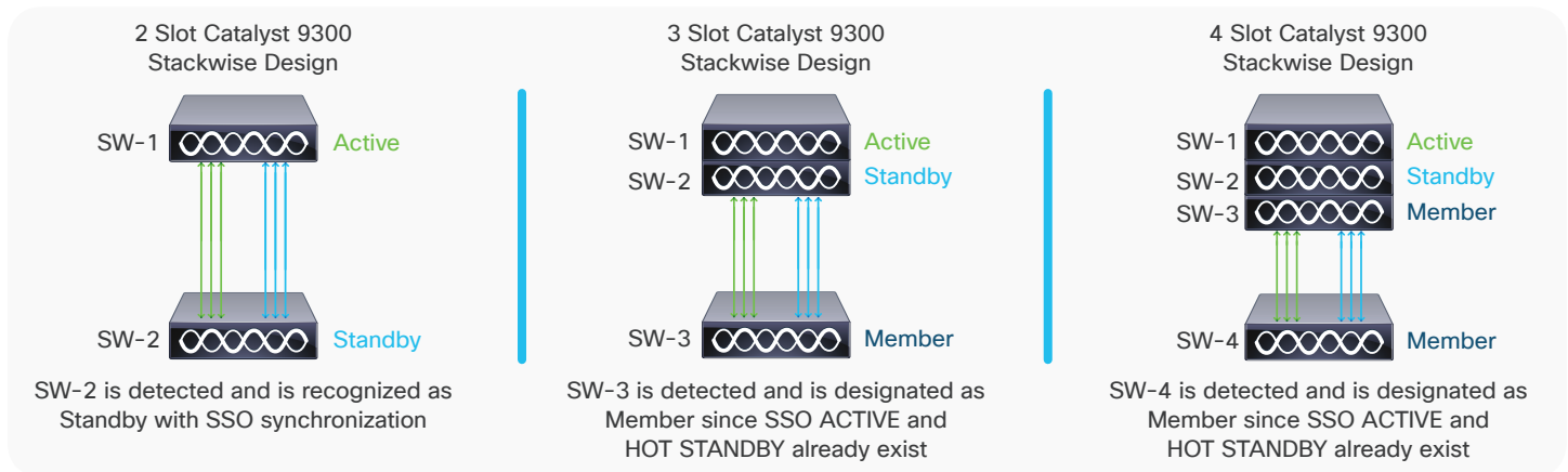
Figure 6. Roles and operation of StackWise-480
