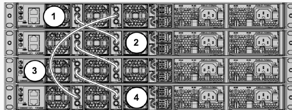
Figure 11. Stack cable connections with four switches in the stack
