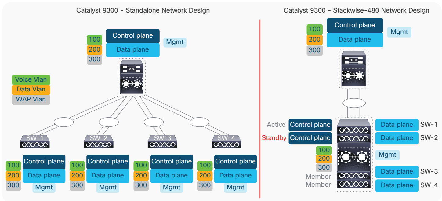
Figure 16. Comparison of Cisco Catalyst 9300 Series Switches in standalone mode to a StackWise-480 multilayer network design
