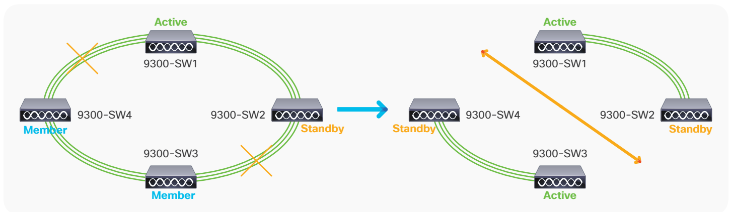
Figure 13. Stack split scenario
