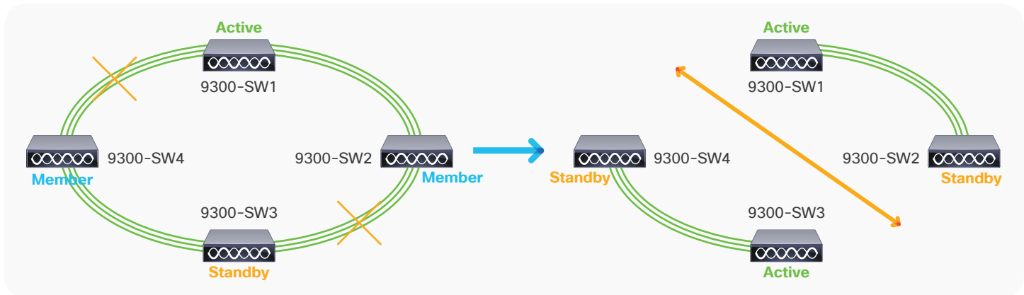
Figure 14. Another stack split scenario
