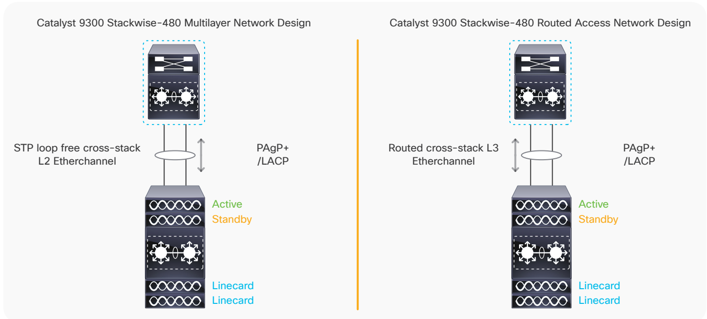
Figure 18. Cisco Catalyst 9300 Series cross-stack EtherChannel design
