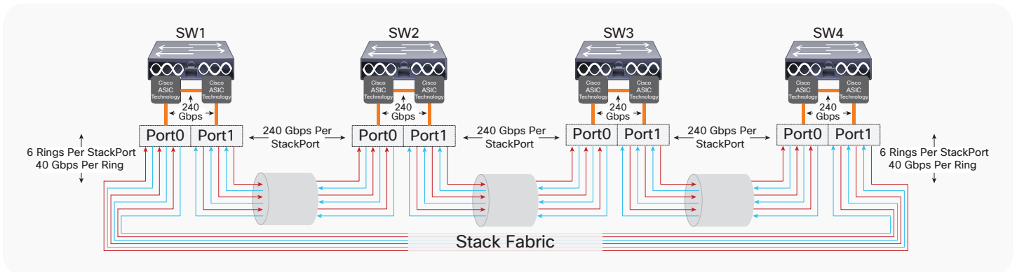
Figure 5. Cisco Catalyst 9300 StackWise-480 internal forwarding architecture
