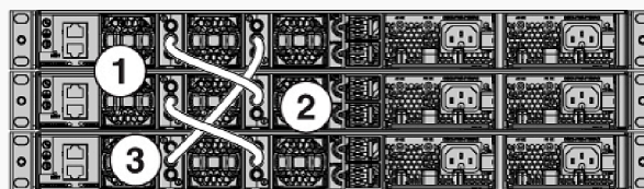
Figure 12. Stack cable connections after switch 4 has been removed from the stack
