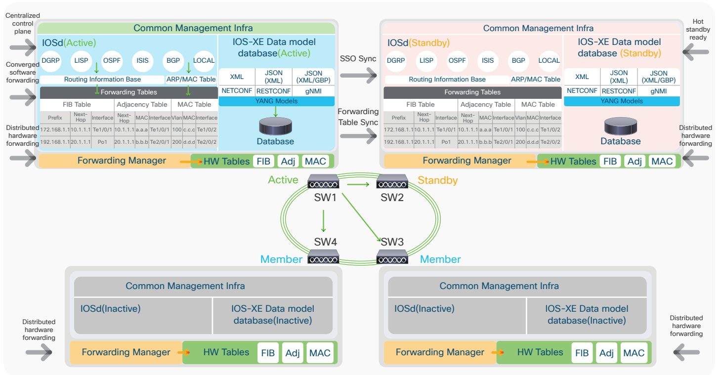
Figure 8. Cisco Catalyst 9300 Series StackWise-480 NSF/SSO architecture
