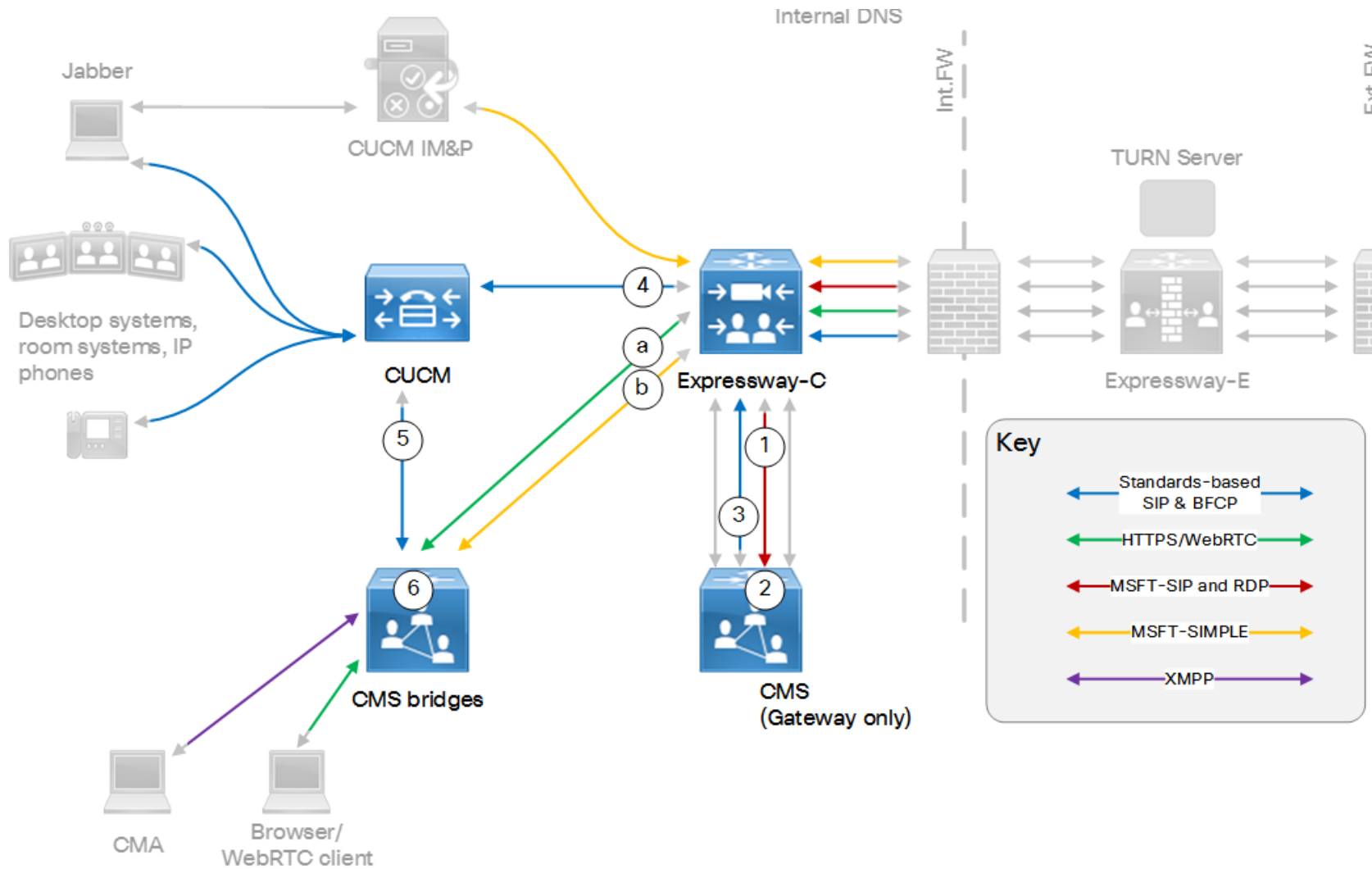
Figure 9 Traffic Routing
