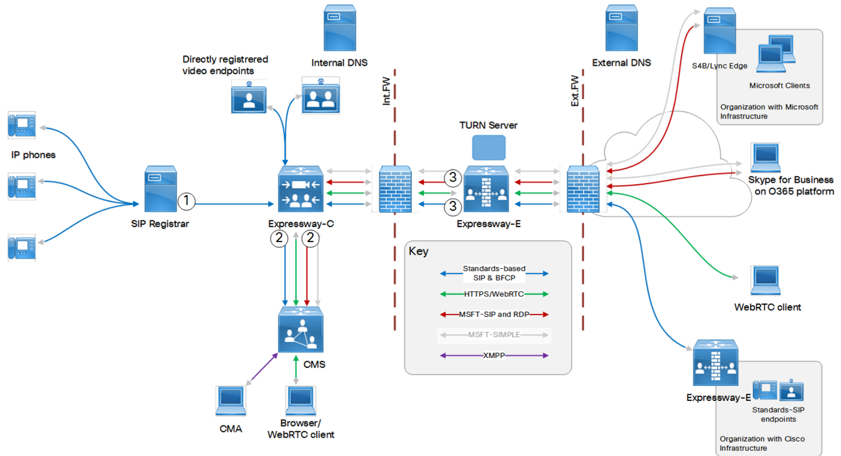
Figure 7 Call Routing
