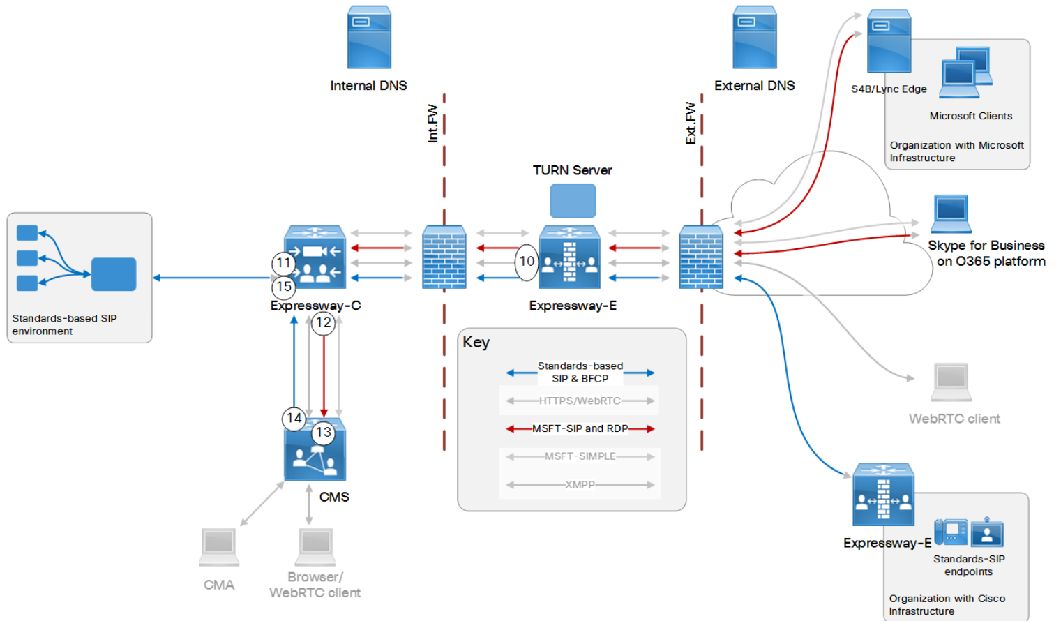
Figure 6 Inbound Call Signaling
