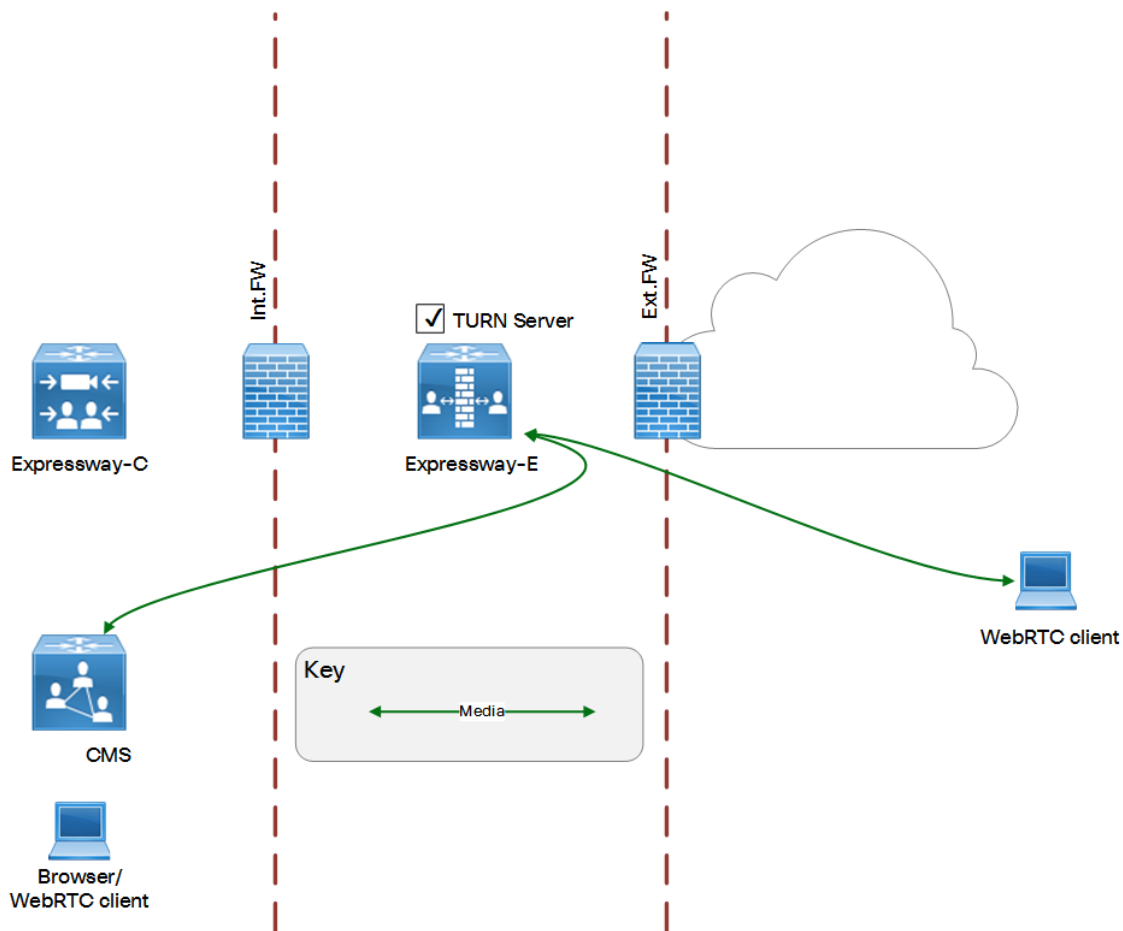
Figure 13 Media Flow Between External WebRTC Client and Meeting Server
