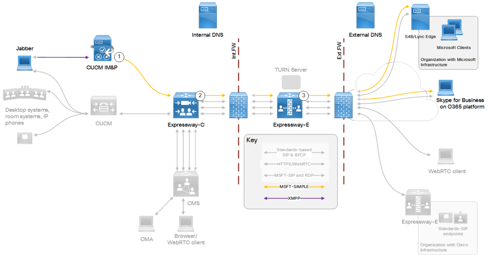
Figure 10 Outbound Signaling
