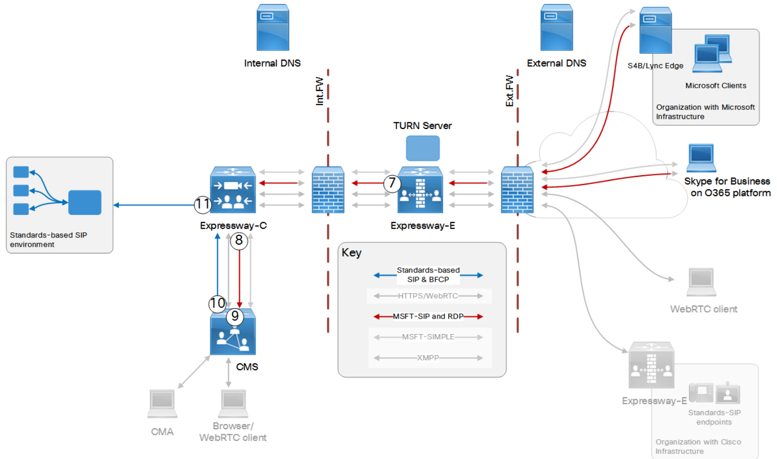
Figure 4 Inbound Call Signaling
