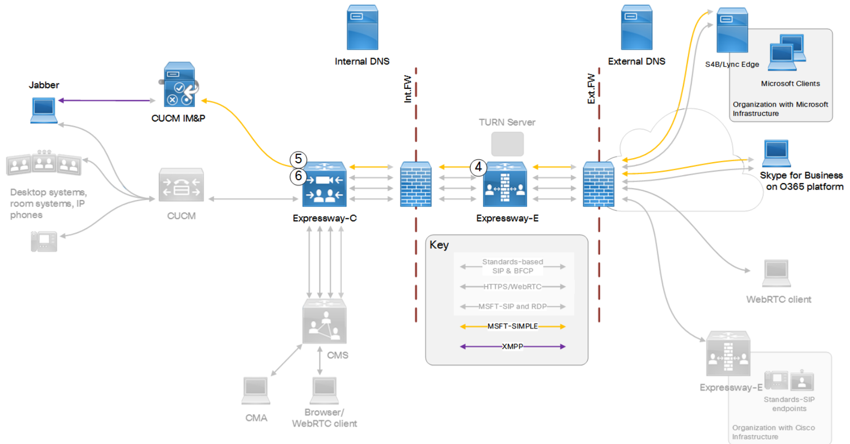
Figure 11 Inbound Signaling
