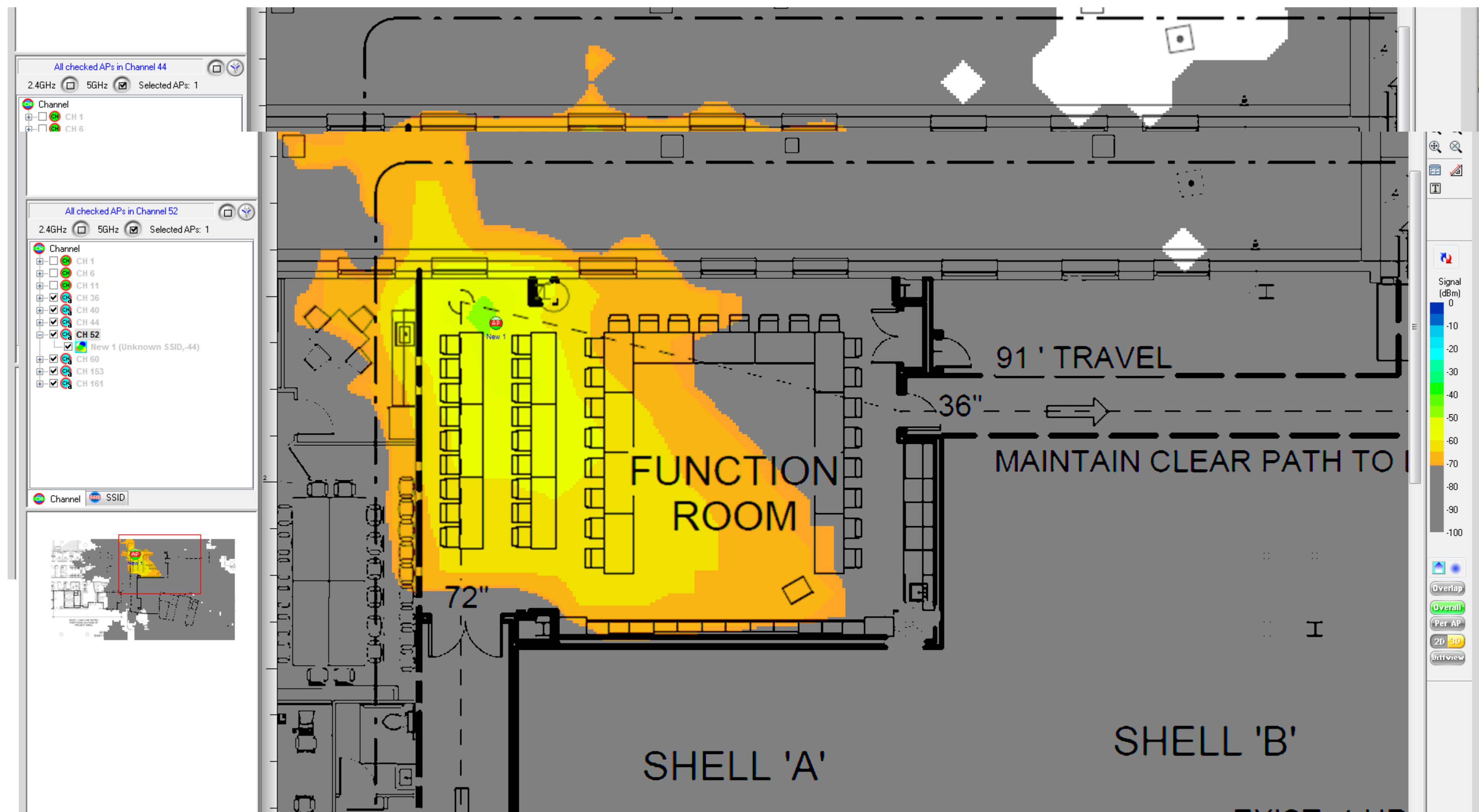
5 GHz AP "New 1" Channel 52 Coverage
