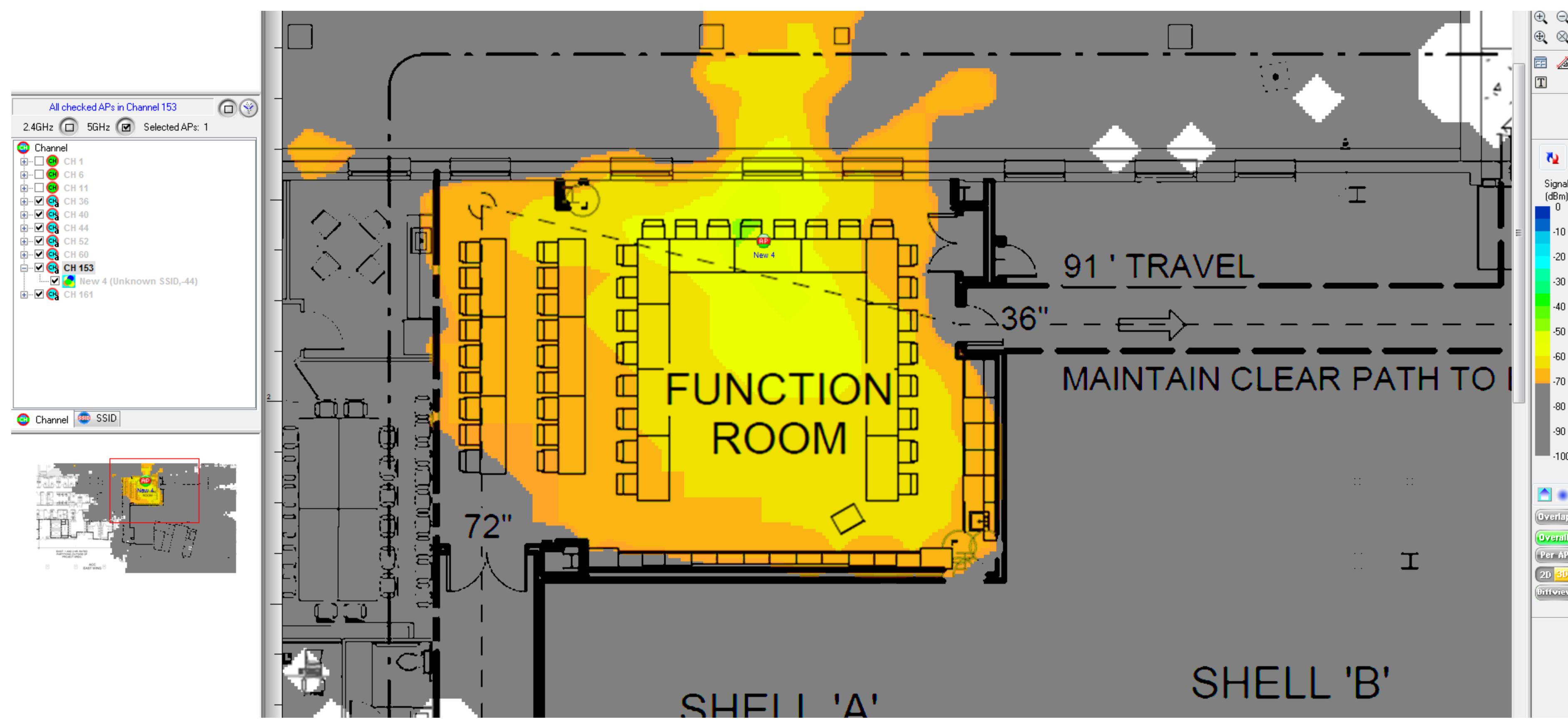
5 GHz AP "New 4" Channel 153 Coverage
