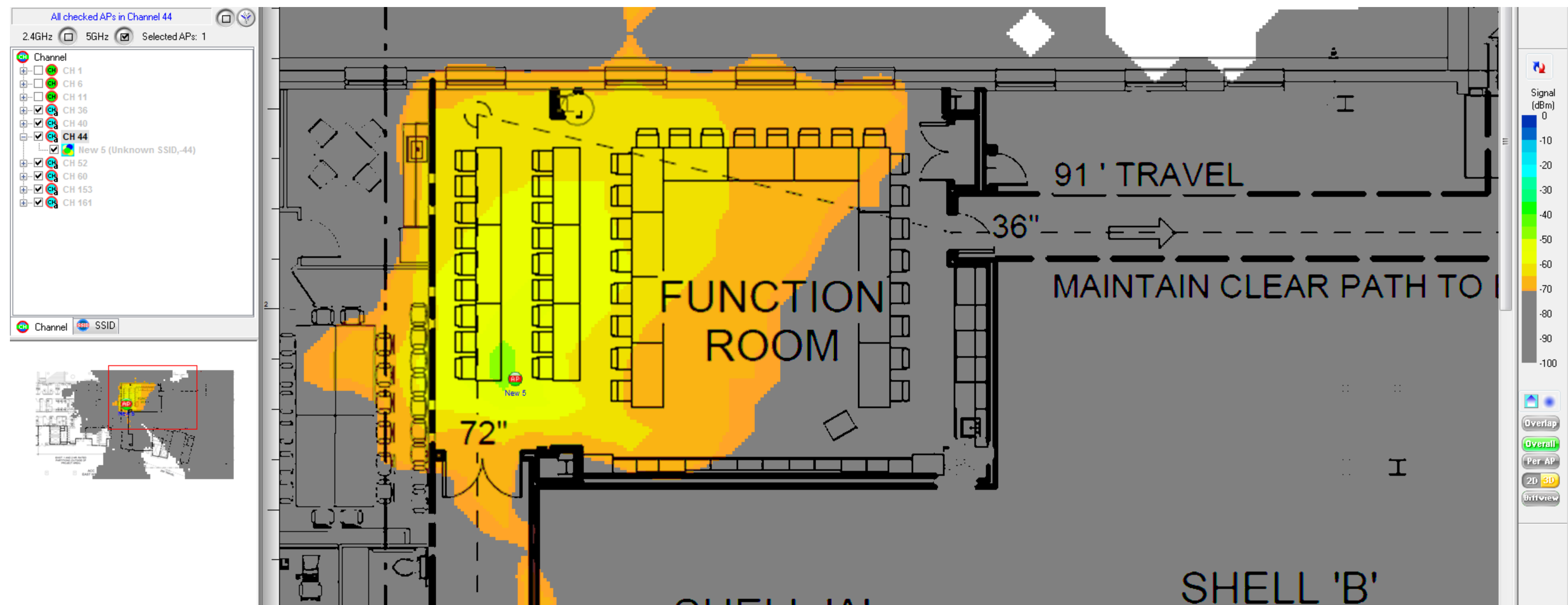
5 GHz AP "New 5" Channel 44 Coverage
