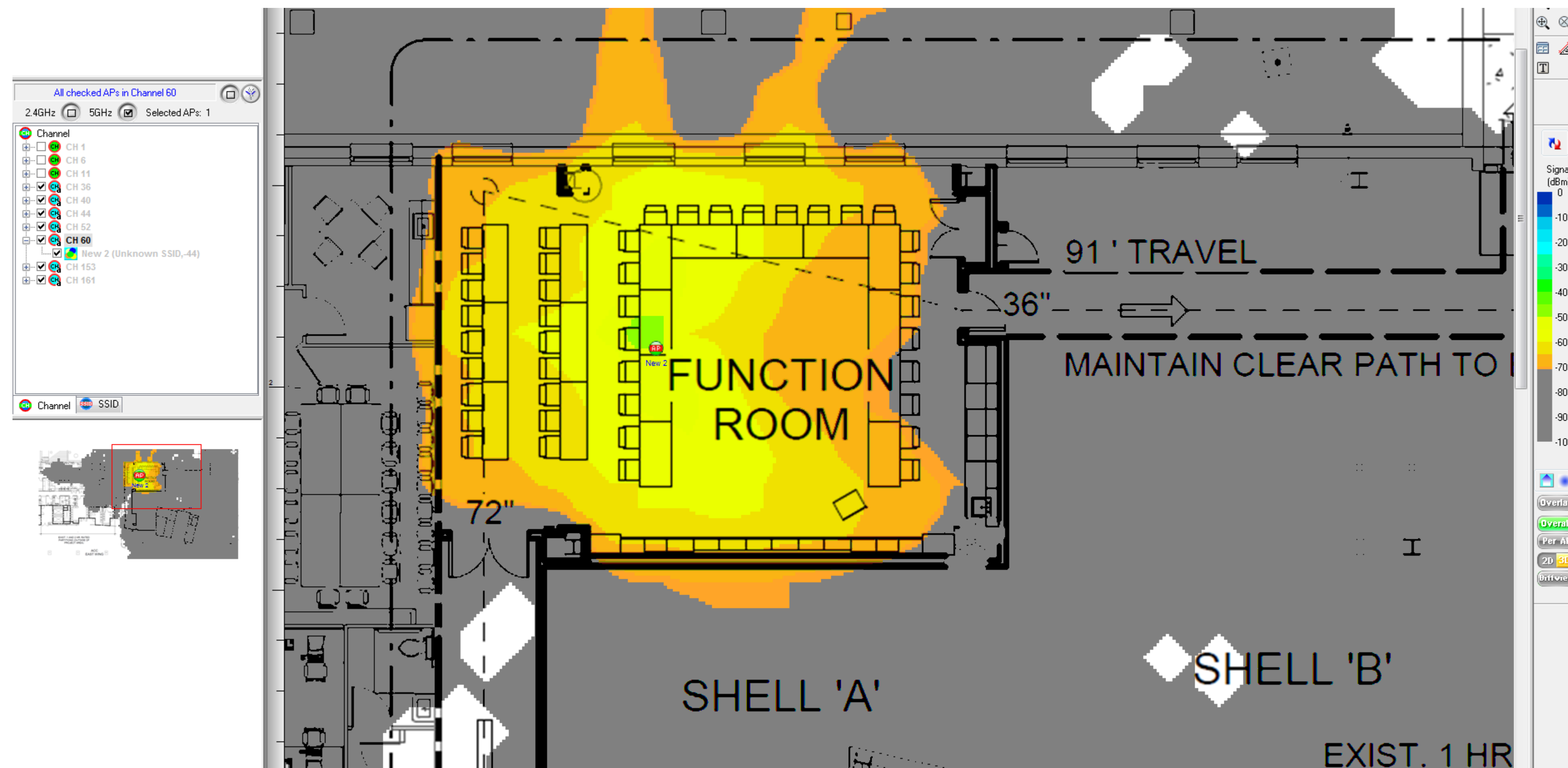
5 GHz AP "New 2" Channel 60 Coverage
