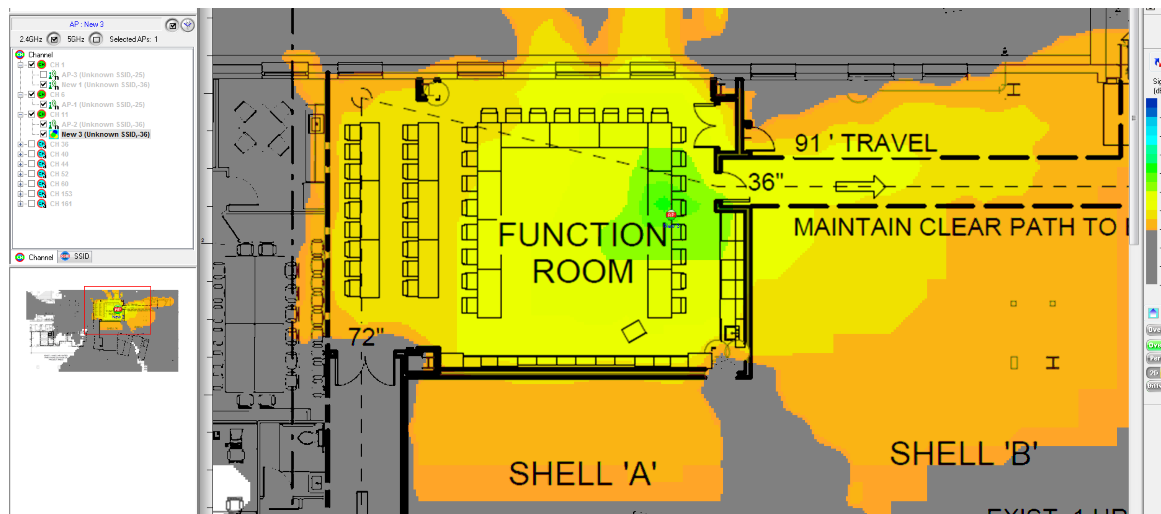
2.4 GHz AP "New 3" Channel 11 Coverage
