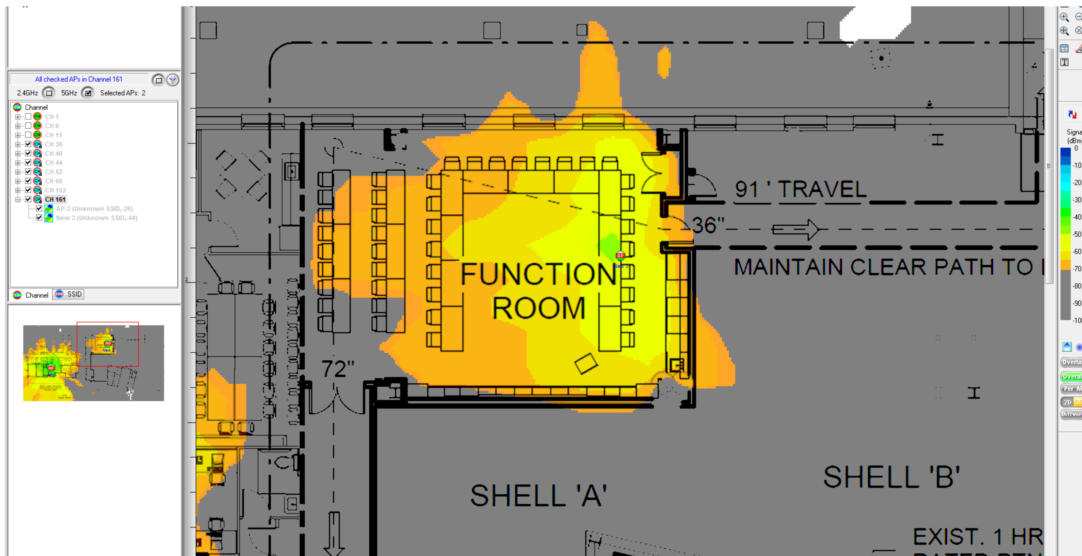
5 GHz AP "New 3" Channel 161 Coverage
